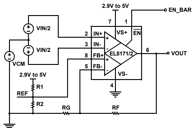
FIGURE 29. CIRCUIT 2 - GAIN SETTING AND REFERENCE CONNECTION
