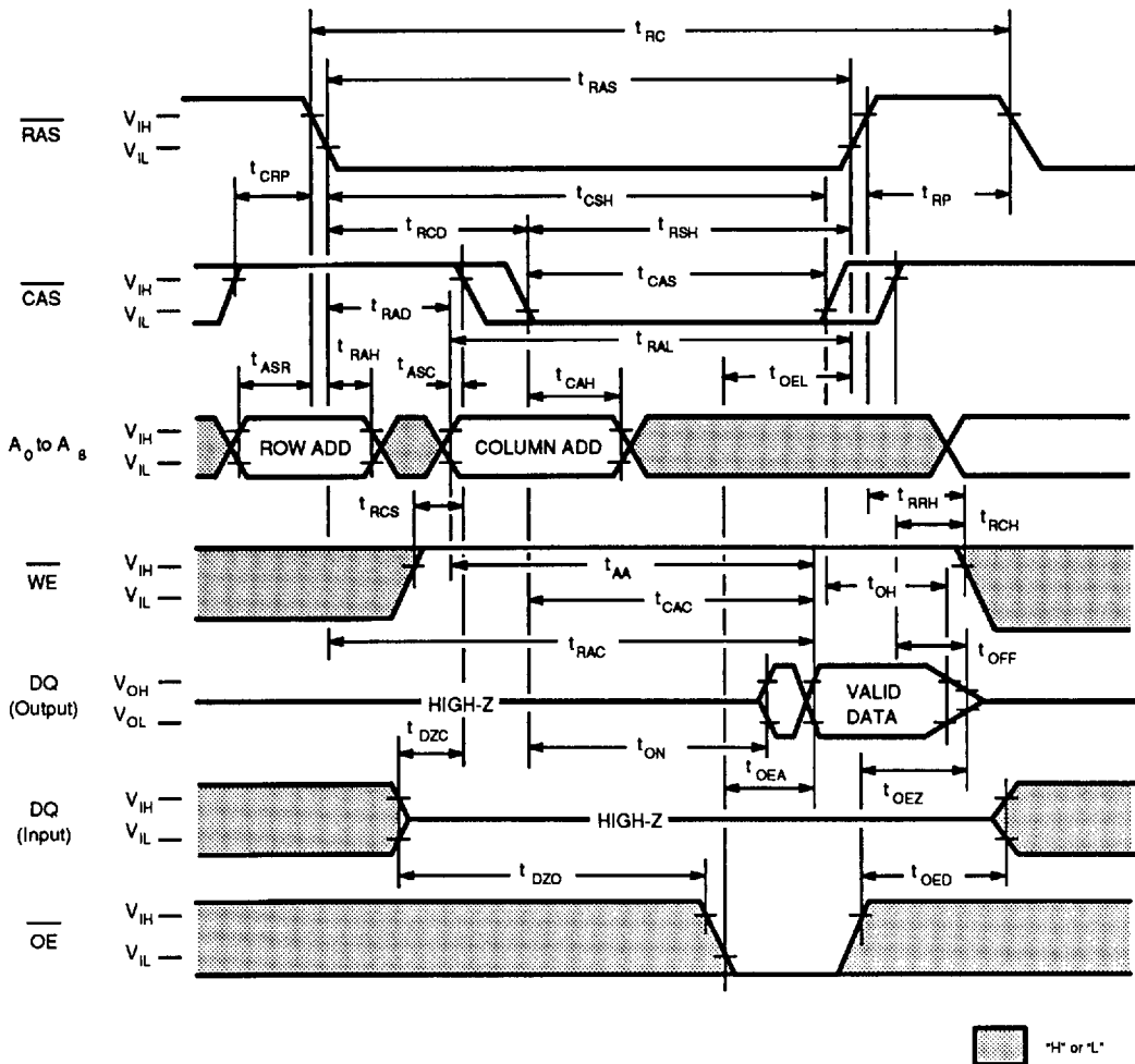
Fig. 4 - READ CYCLE
