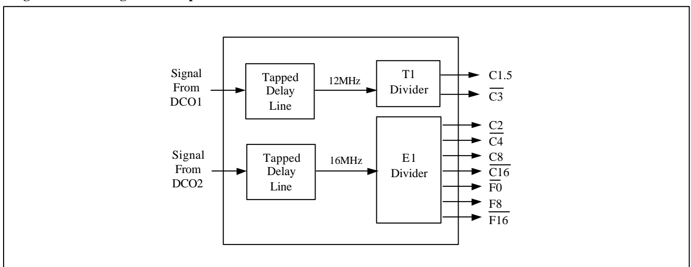
Figure 5. Block Diagram of Output Interface Circuit
