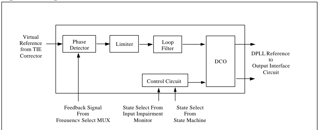
Figure 4. Block Diagram of DPLL
