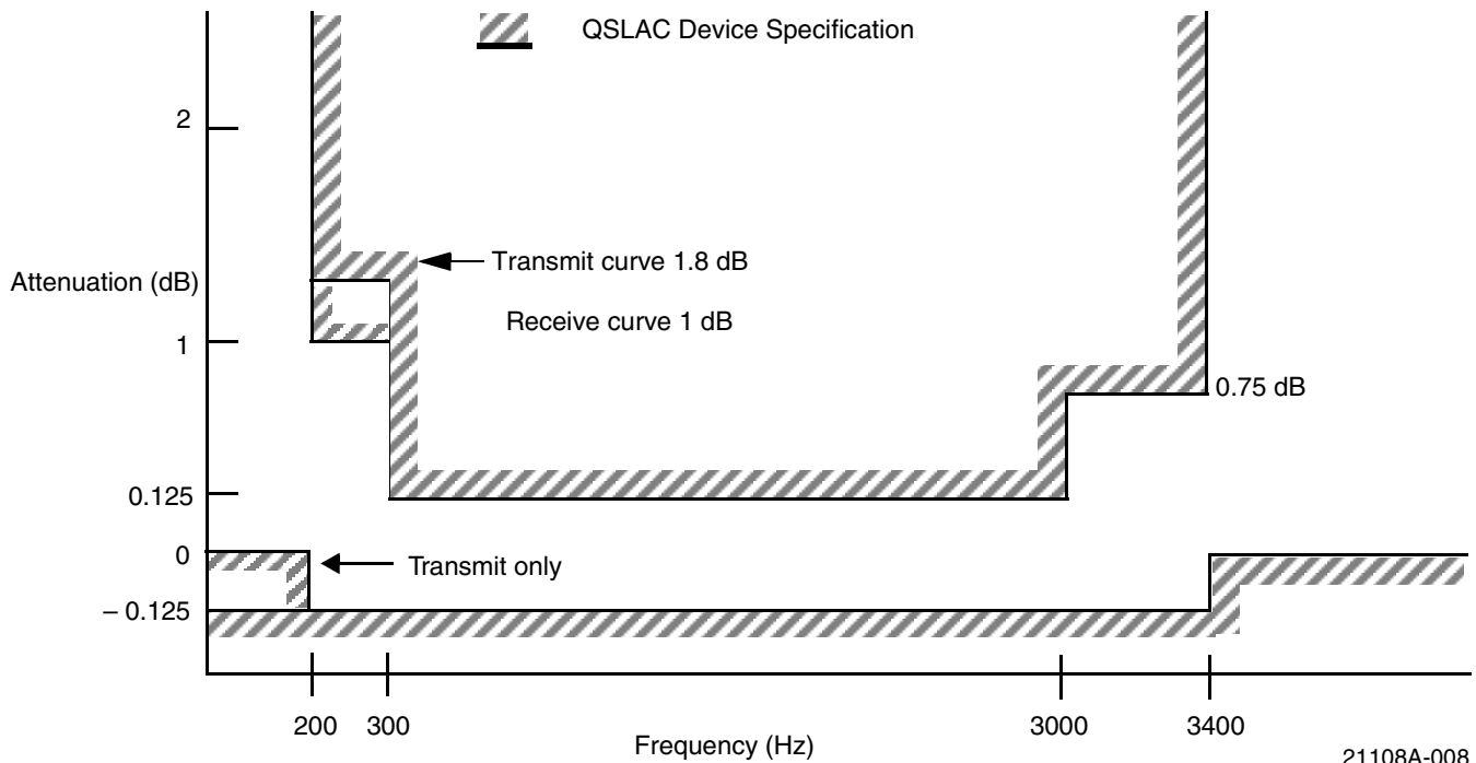
Figure 1. Attenuation Distortion
