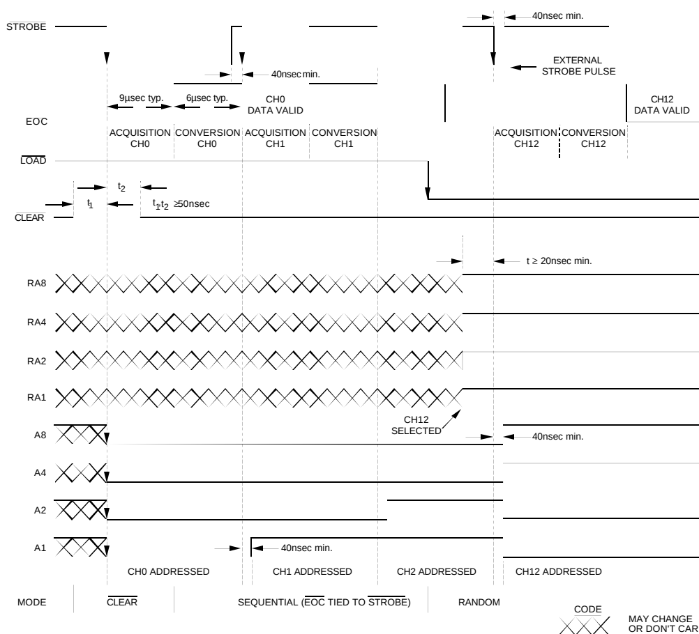
Figure 4. HDAS Timing Diagram
