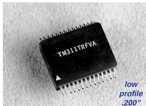
Model TM311TRFVA for AMCC S3015/S3016 or S3031B chip sets. Contains loss-of-signal (LOS) detection circuit.
