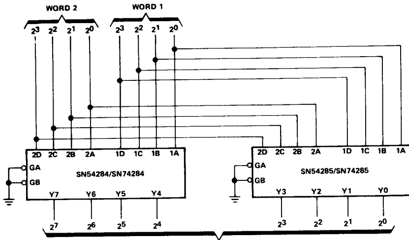
FIGURE A-4 X 4 MULTIPLIER
