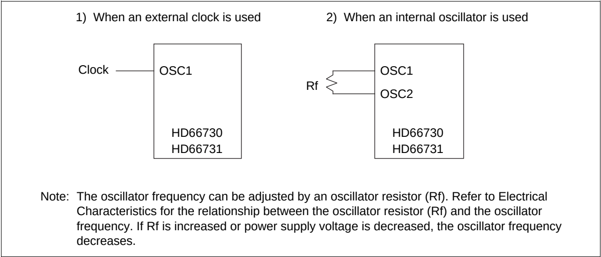
Figure 41 Oscillator Connections
