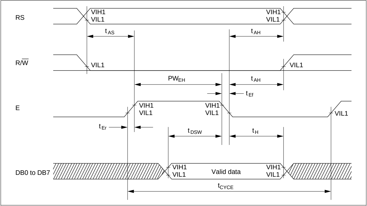
Figure 50 Bus Write Operation
