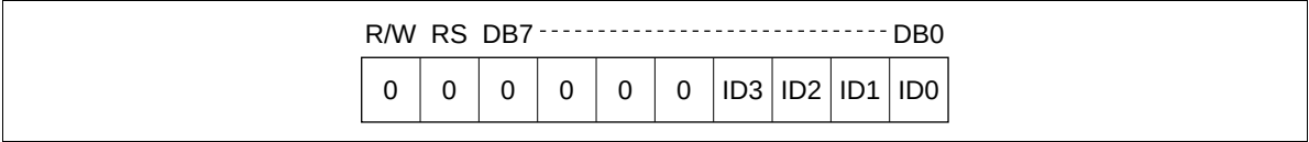
Figure 4 Index Register
