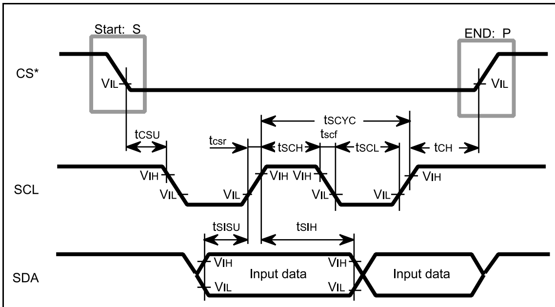
Figure 42 Clock-Synchronized Serial Interface Timing
