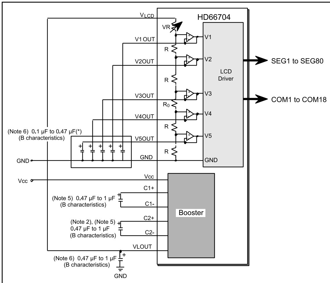
Figure 25 Internal Booster Circuit for LCD Drive Voltage Generation
