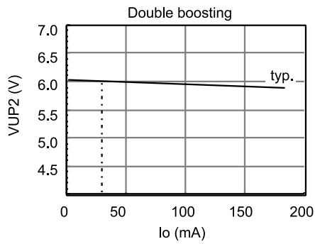
Figure 40 Booster (cont)
