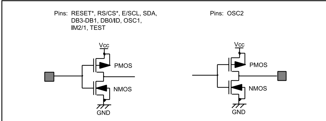
Figure 36 I/O Pin Configuration
