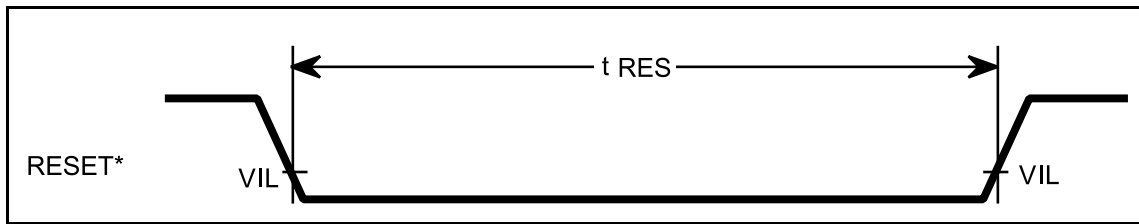
Figure 43 Reset Timing
