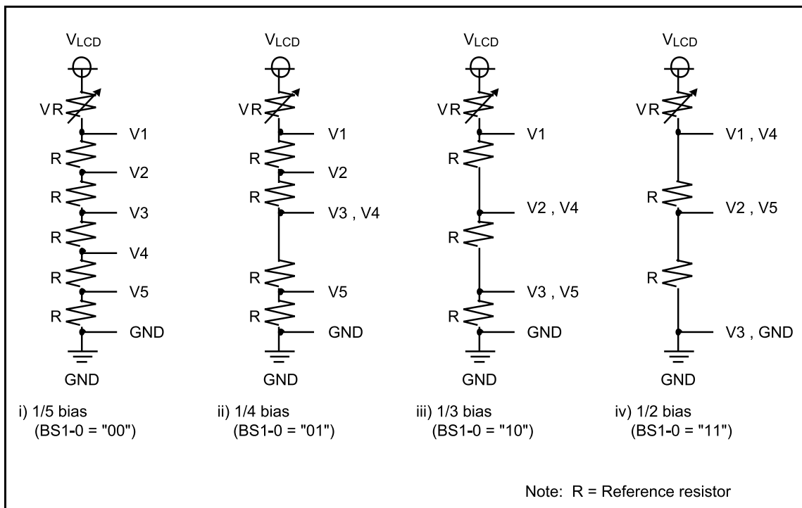
Figure 26 Liquid Crystal Display Drive Bias Circuit
