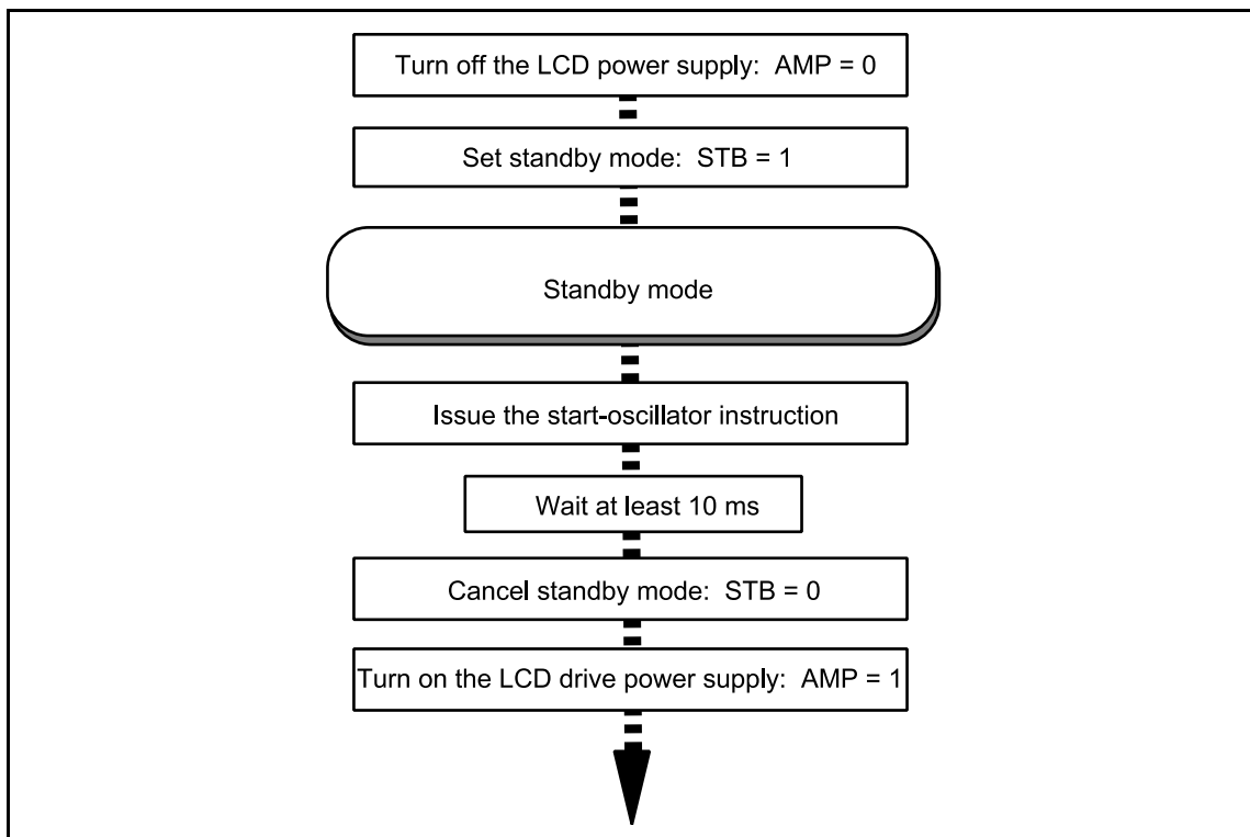
Figure 35 Procedure for Setting and Canceling Standby Mode
