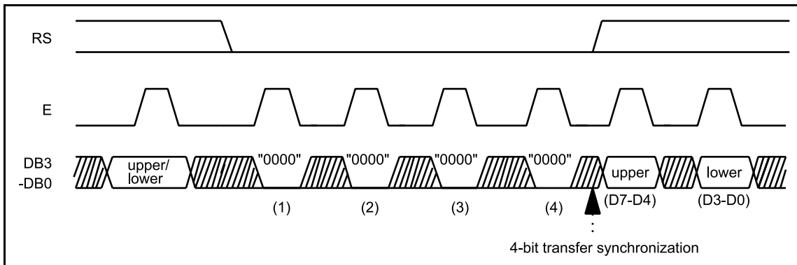
Figure 21 4-Bit Transfer Synchronization
