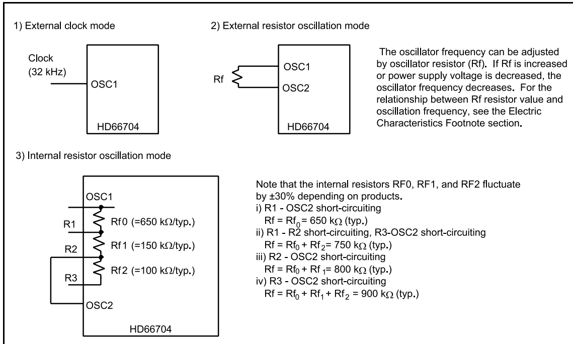
Figure 22 Oscillator Circuits
