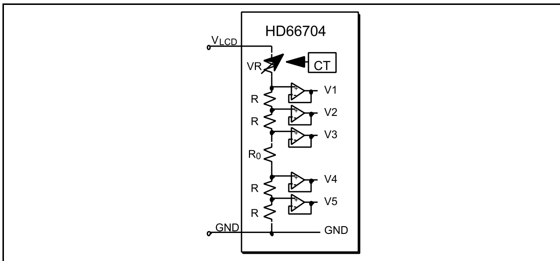
Figure 27 Contrast Adjuster
