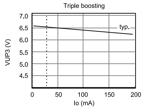
Figure 40 Booster (cont)
