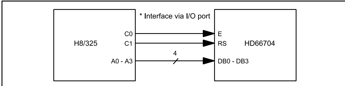
Figure 20 Interface to 4-Bit Microcomputer
