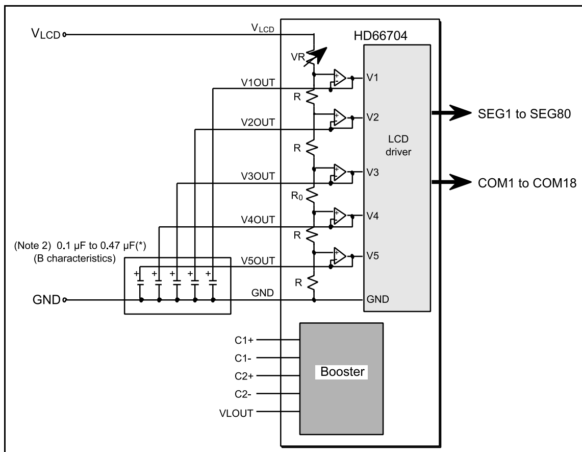
Figure 24 External Power Supply Circuit for LCD Drive Voltage Generation
