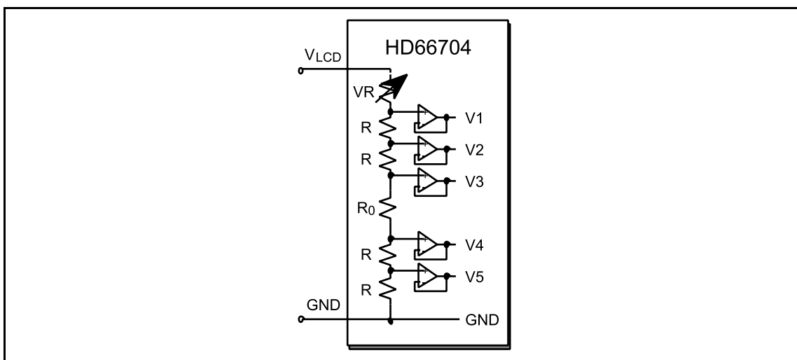
Figure 9 Contrast Adjuster
