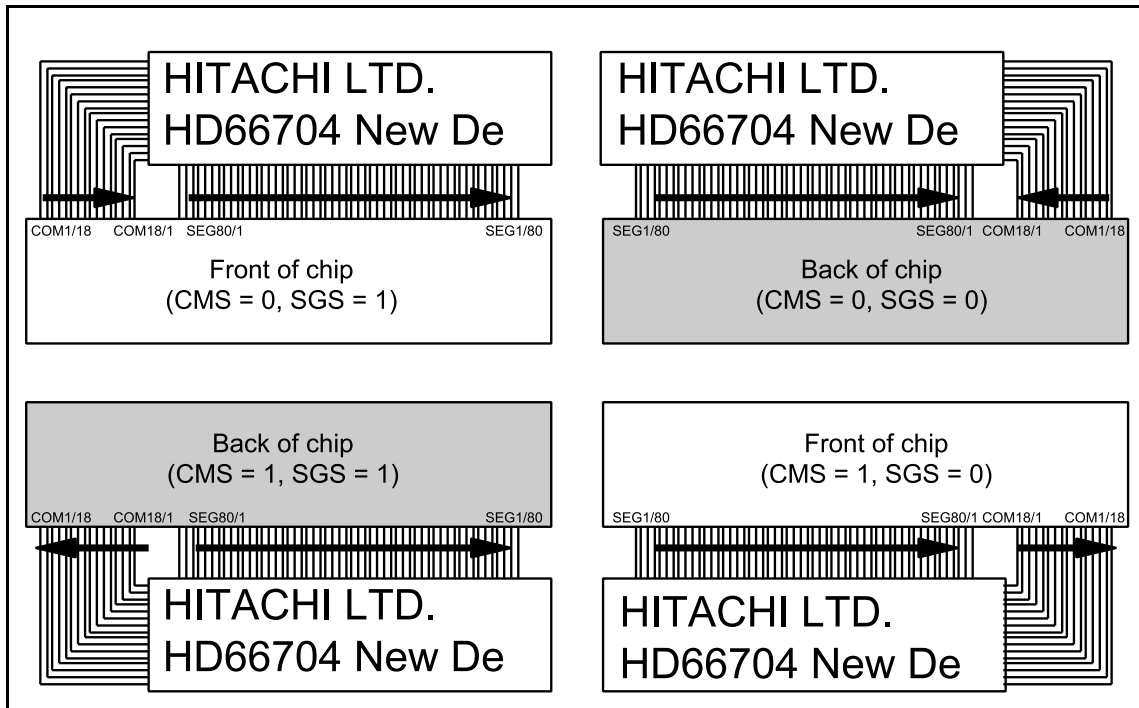
Figure 28 Pattern Wiring for 2-Line Character Display
