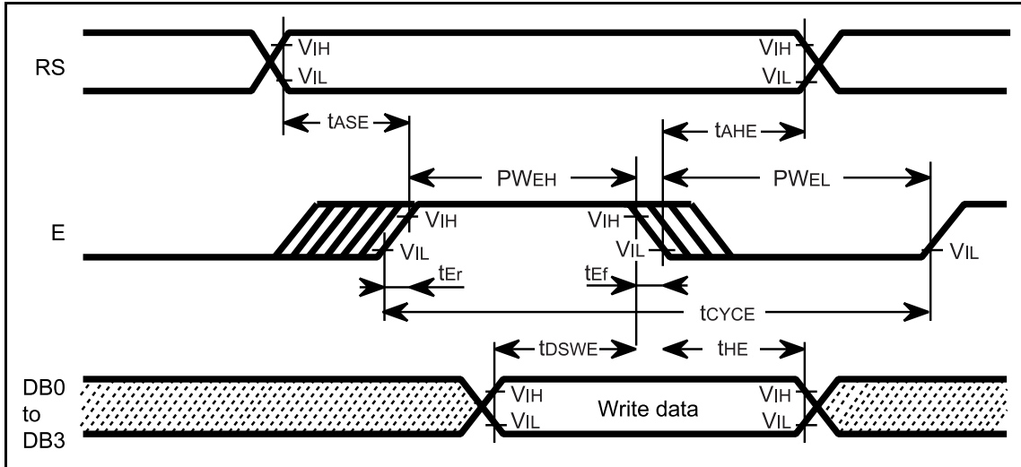
Figure 41 4-Bit Bus Timing
