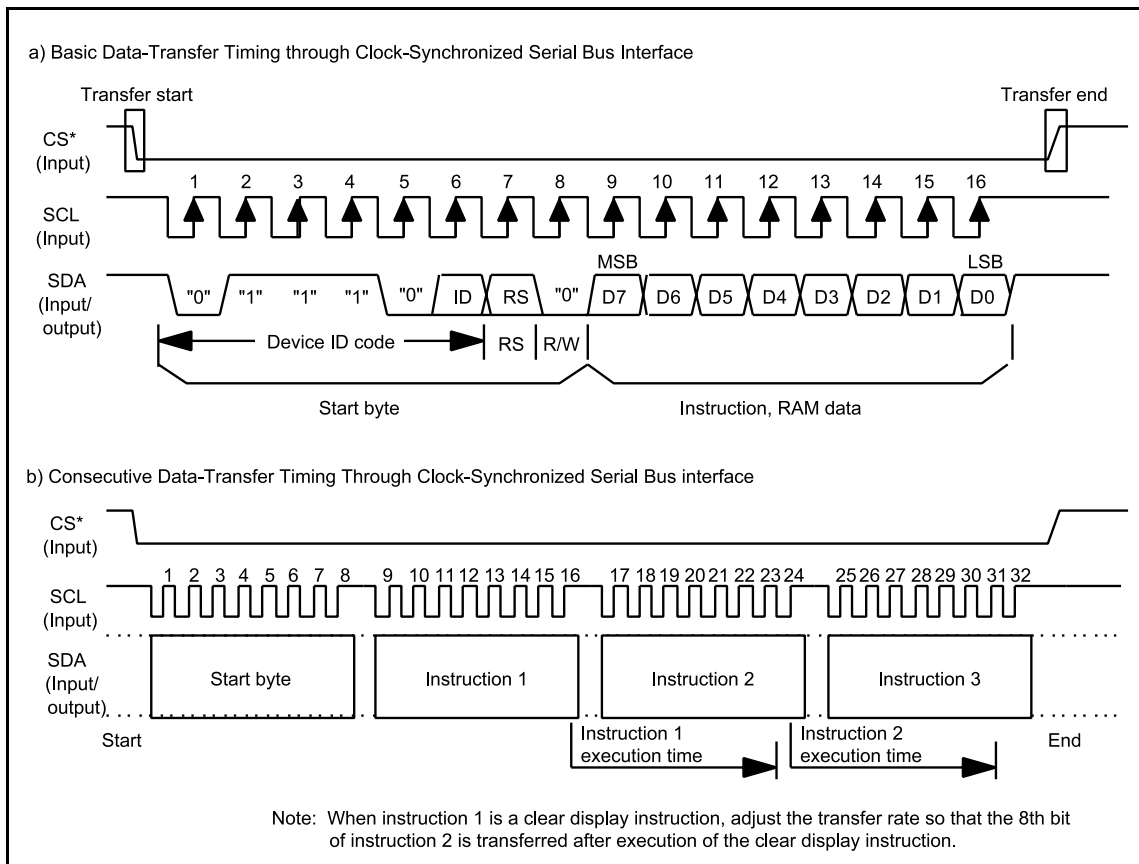
Figure 19 Clock-Synchronized Serial Interface Timing Sequence
