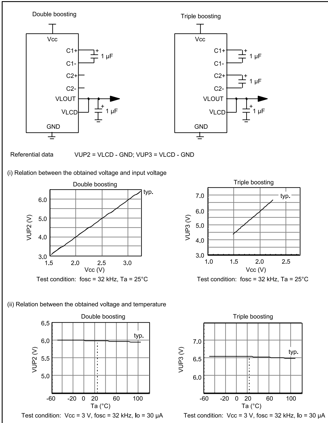
Figure 40 Booster
