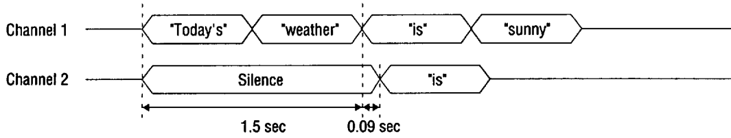
Figure 6 Playback Timing Using Table 14 Edit Data
