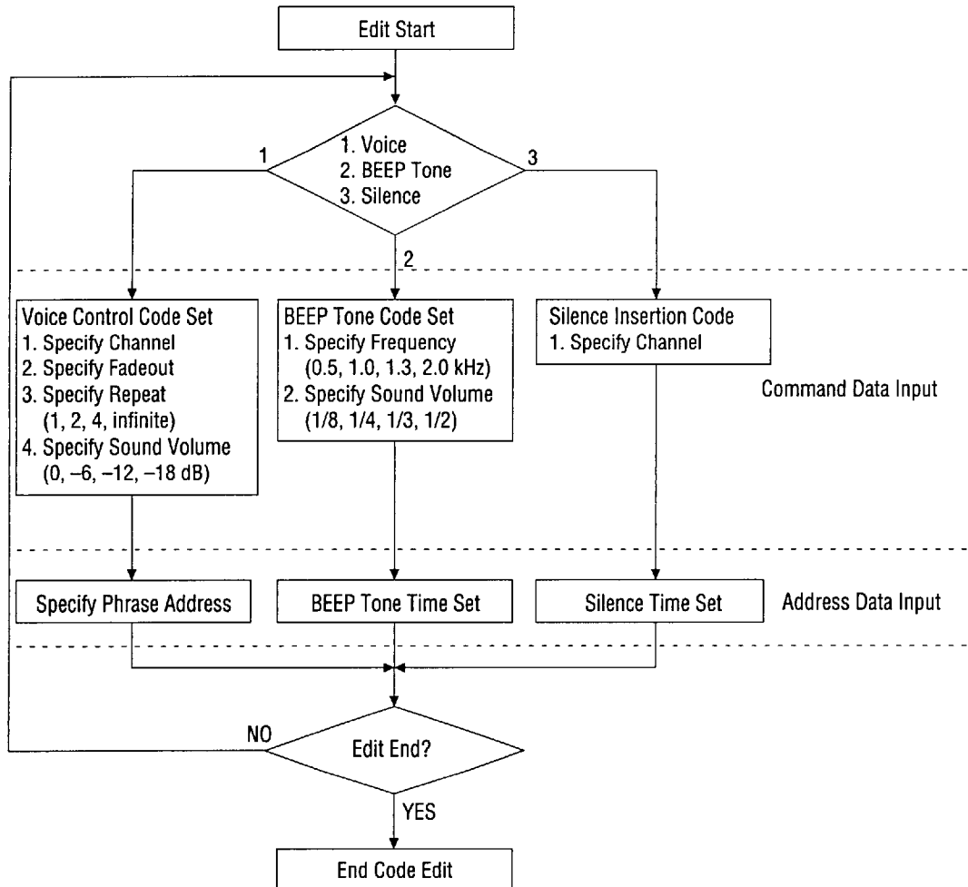
Figure 1 Edit Data ROM Flowchart
