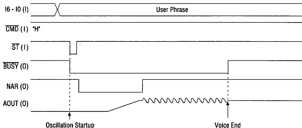
Figure 7.1 Voice Startup Timing
