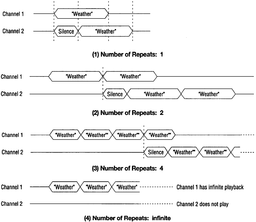
Figure 3 Echo Playback Timing Using Repeated Playback
