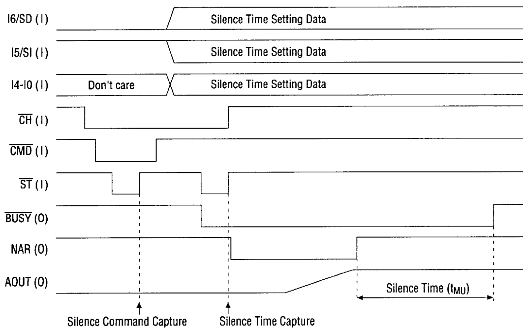
Figure 6.2 Channel 2 Silence Set Timing (Parallel Input)
