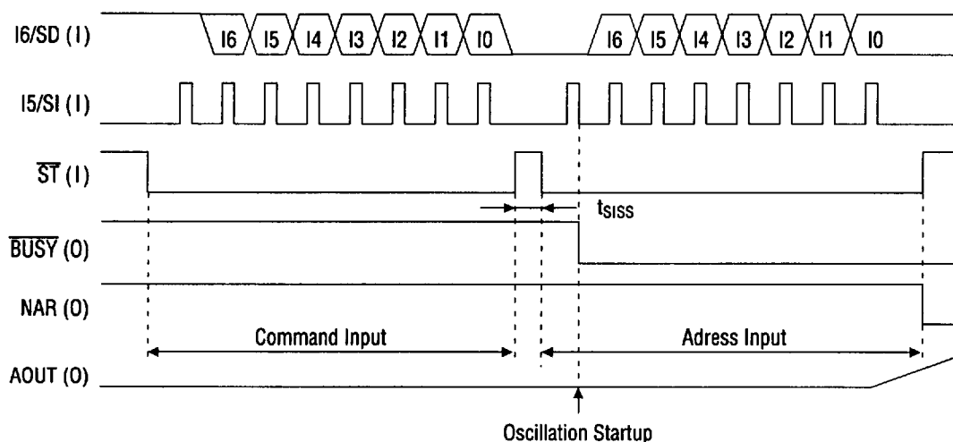
Figure 5.2 Command, Address Input Timing (Serial Input)
