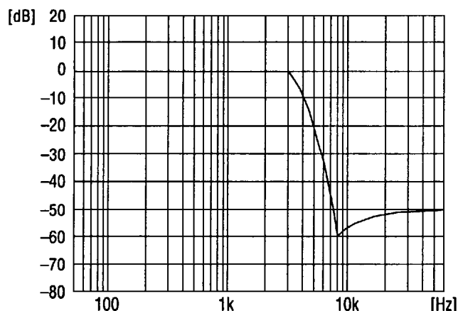
Figure 14.1 LPF Frequency Characteristics ( f_s = 8.0 kHz)
