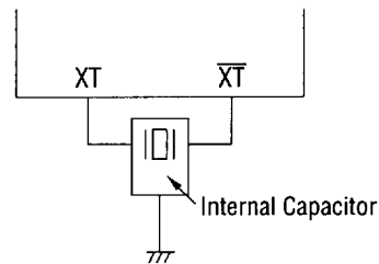
Figure 14.3 CST4.09MGWU
