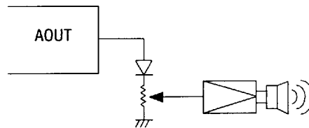
Figure 15.2 Pop Noise Killer Circuit
