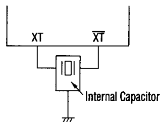
Figure 16.3 CST4.09MGWU
