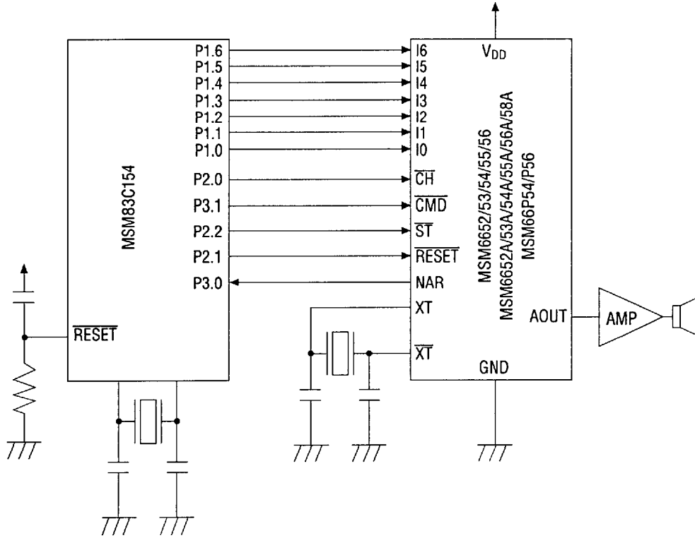
Application circuit in Parallel Input Interface Mode
