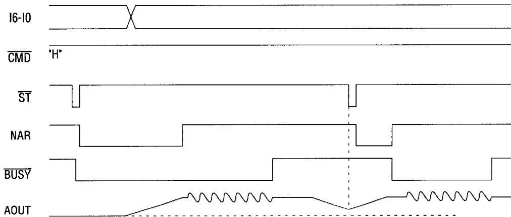
Figure 13.1 \overline{\text{ST}} Pulse Input Timing during Standby Conversion
