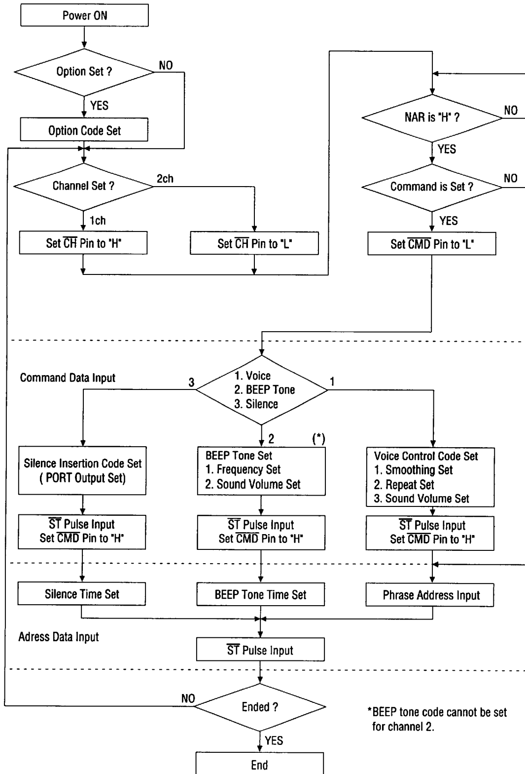
Figure 5.4 Parallel Input Flowchart when External Command is Used
