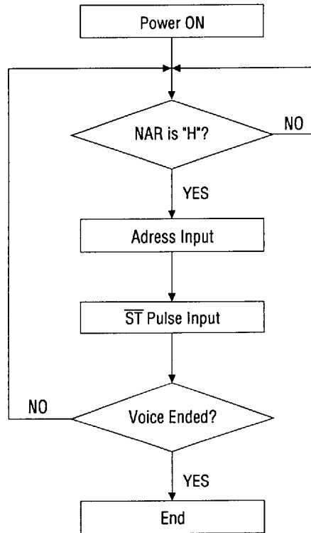
Figure 5.3 Input Flowchart when Command is Not Set
