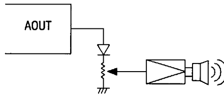
Figure 12.2 Pop Noise Killer Circuit
