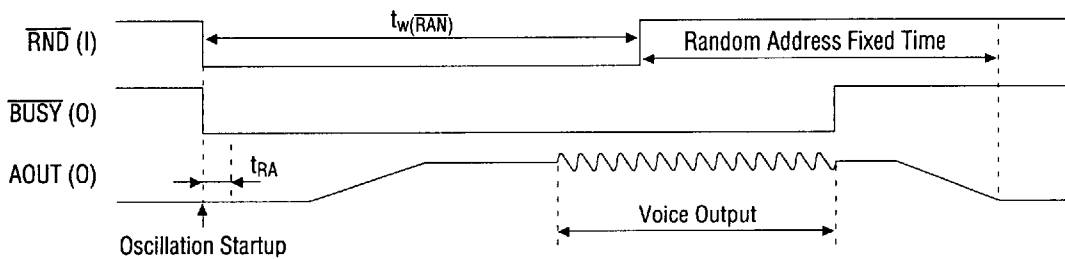
Figure 5.6 Random Address Capture
