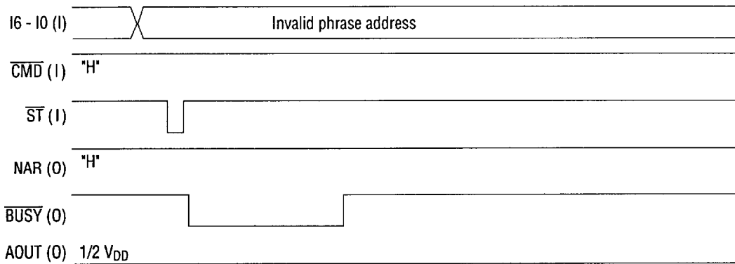
Figure 7.3 Timing when Address, Other than a Phrase, is Input when AOUT is 1/2 V_{DD}
