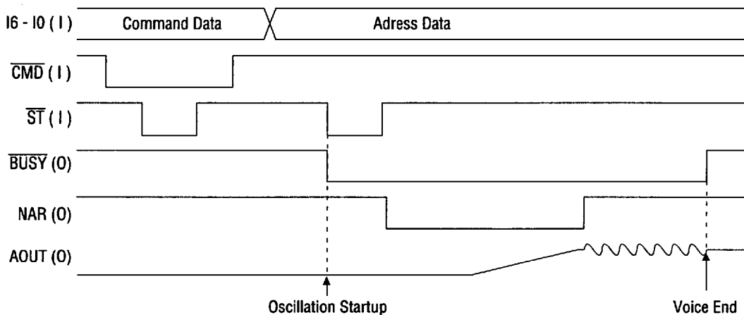
Figure 5.1 Command, Address Input Timing (Parallel Input)
