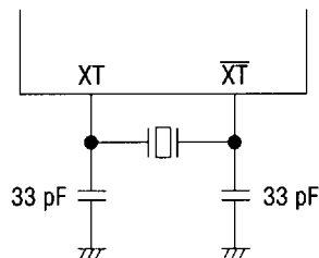
Figure 14.4 PBRC4.00MSA/MKS/MWS
