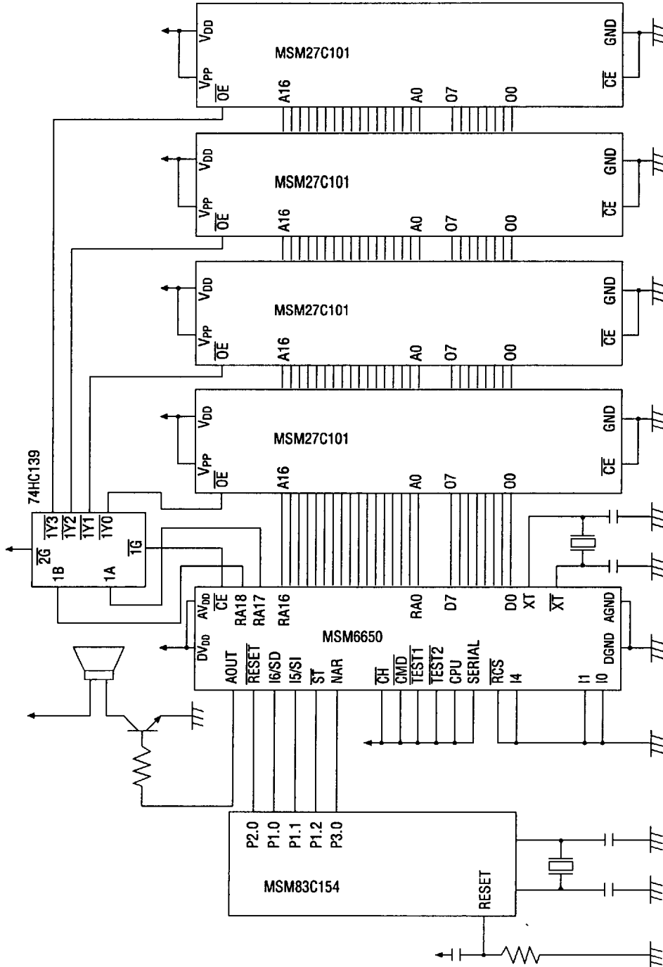
Application Circuit in Microcontroller Interface Mode Using Four 1-Mbit EPROMs (Serial Input Interface)
