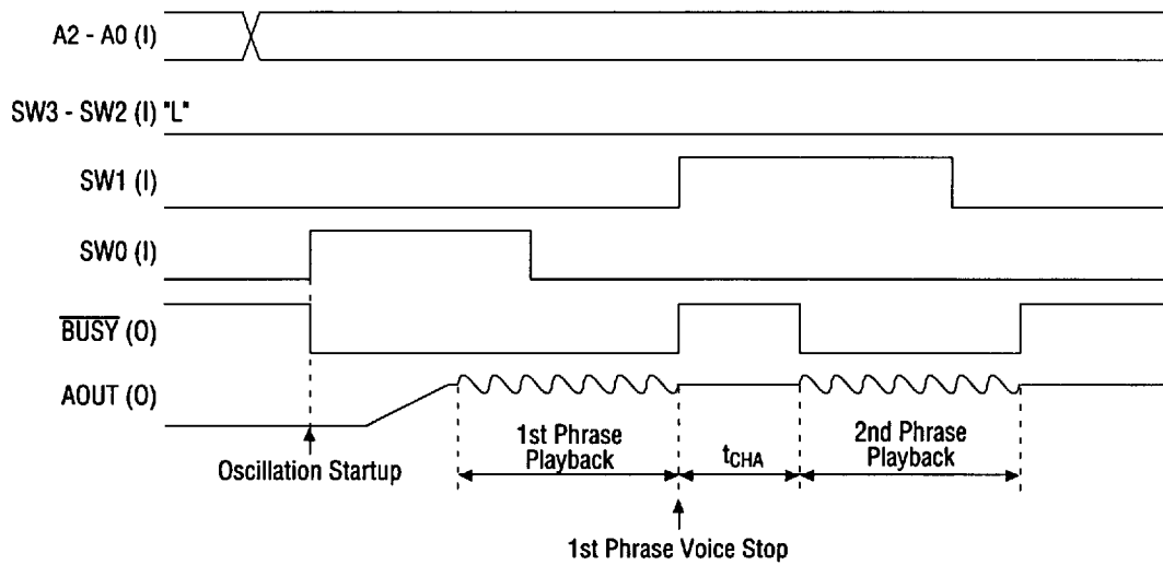
Figure 5.4 Timing when SW3-SW0 are Changed during Playback
