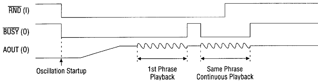
Figure 5.8 Repeat Playback Timing of Random Play
