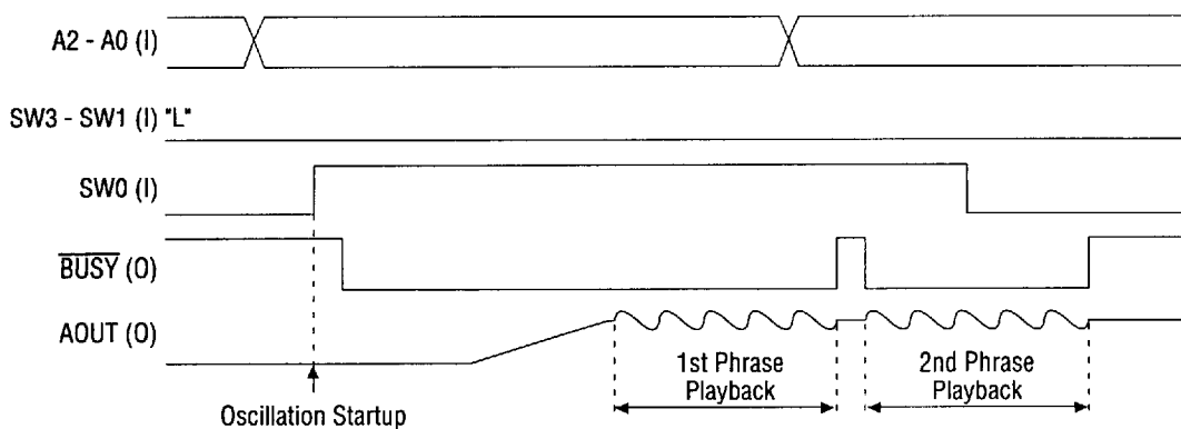
Figure 5.3 SW Input Interface Playback Timing
