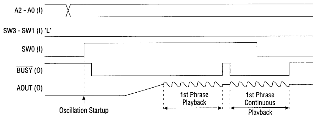
Figure 5.2 SW Input Interface – Repeated Playback Timing
