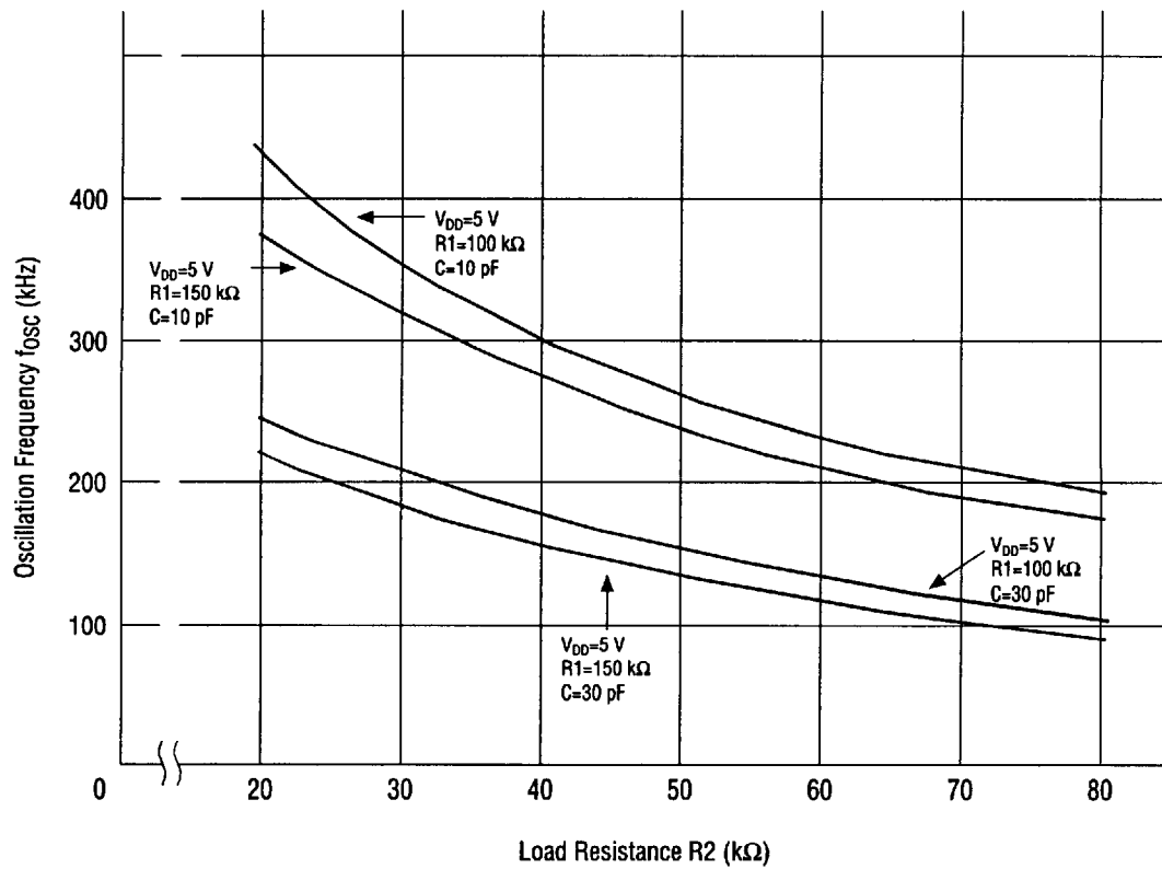
Figure 13.4 RC Oscillation Frequency Characteristics (MSM6650)
