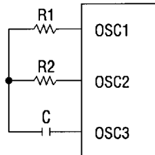
Figure 13.1 RC Oscillation
