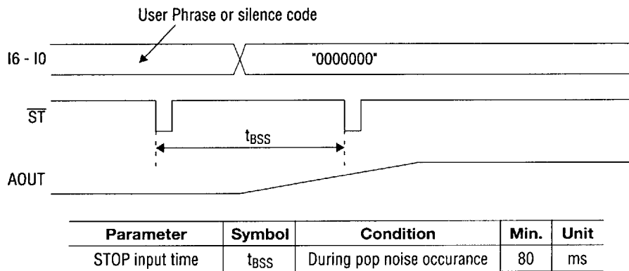
Figure 8.1 STOP Code Input Timing
