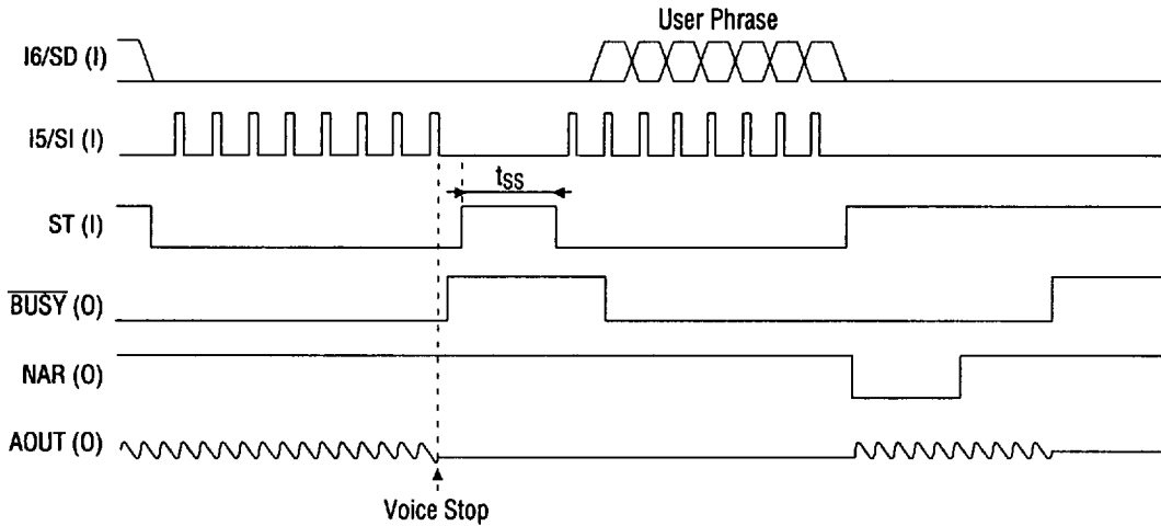
Figure 8.3 STOP Code Input Timing (at Serial Input)
