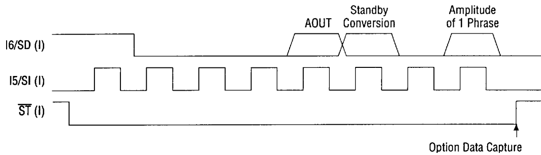
Figure 4.2 Option Set Timing (during Serial Input)
