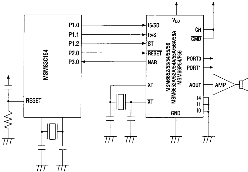
Application Circuit in Serial Input Interface Mode
