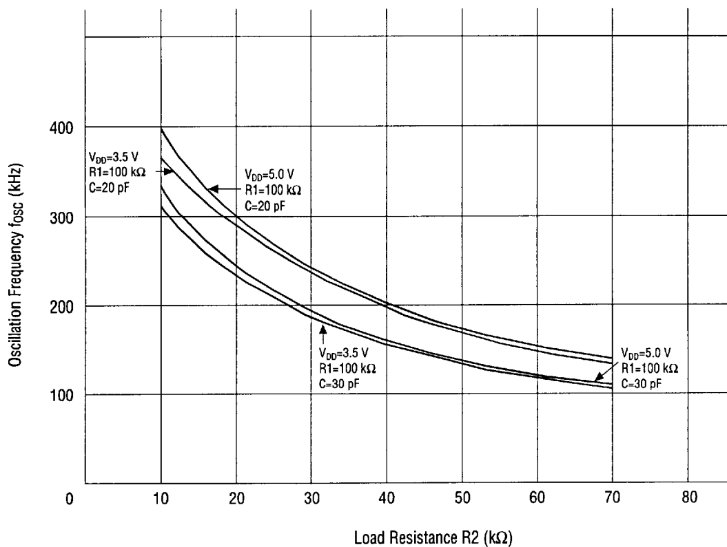
Figure 13.3 RC Oscillation Frequency Characteristics (MSM66P54/P56)
