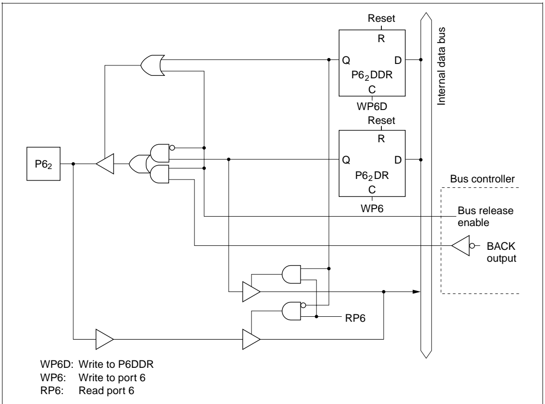
Figure C.2 (c) Port 6 Block Diagram (Pin P6 2 )
