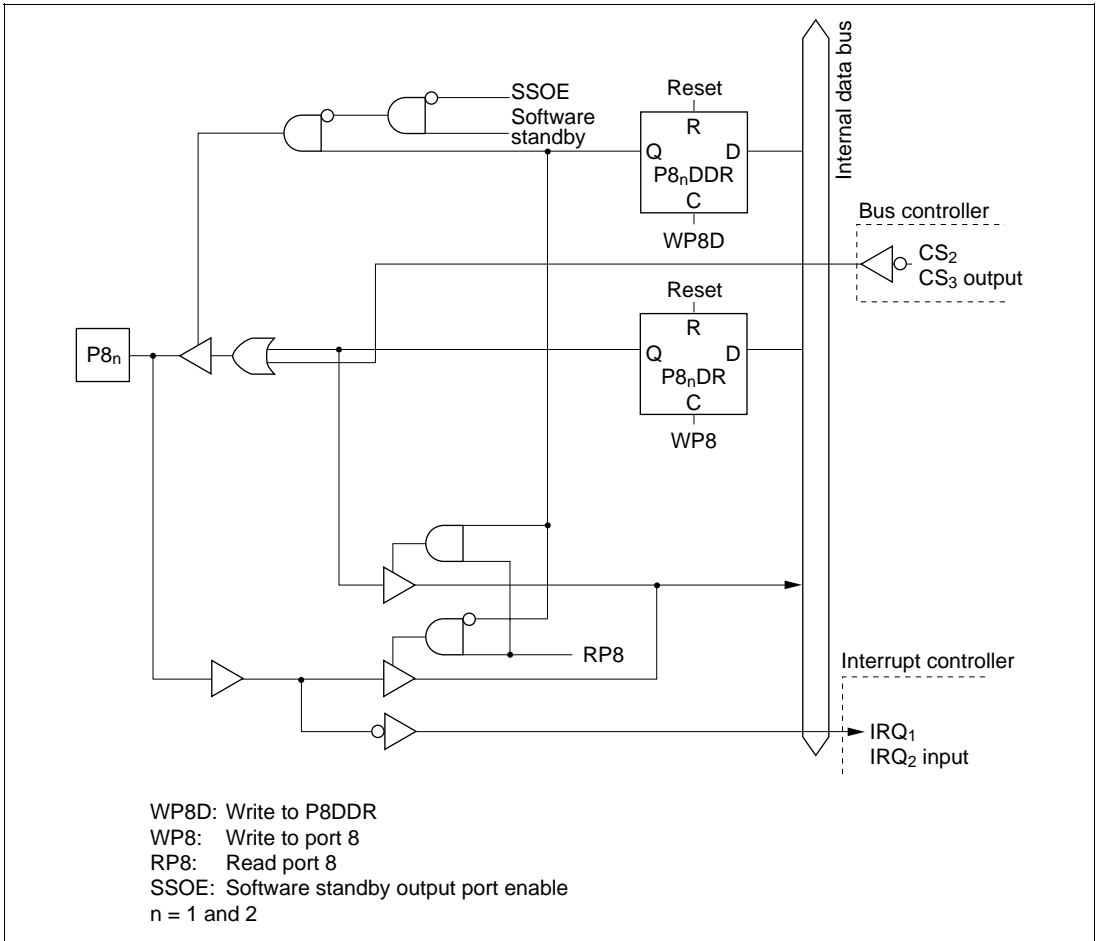
Figure C.4 (b) Port 8 Block Diagram (Pins P8_1 , P8_2 )
