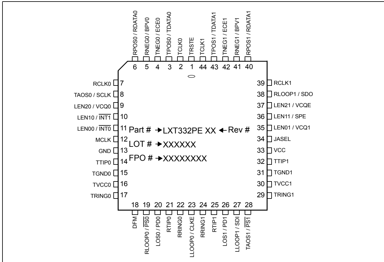
Figure 2 Pin Assignments and Package Markings (PLCC)
