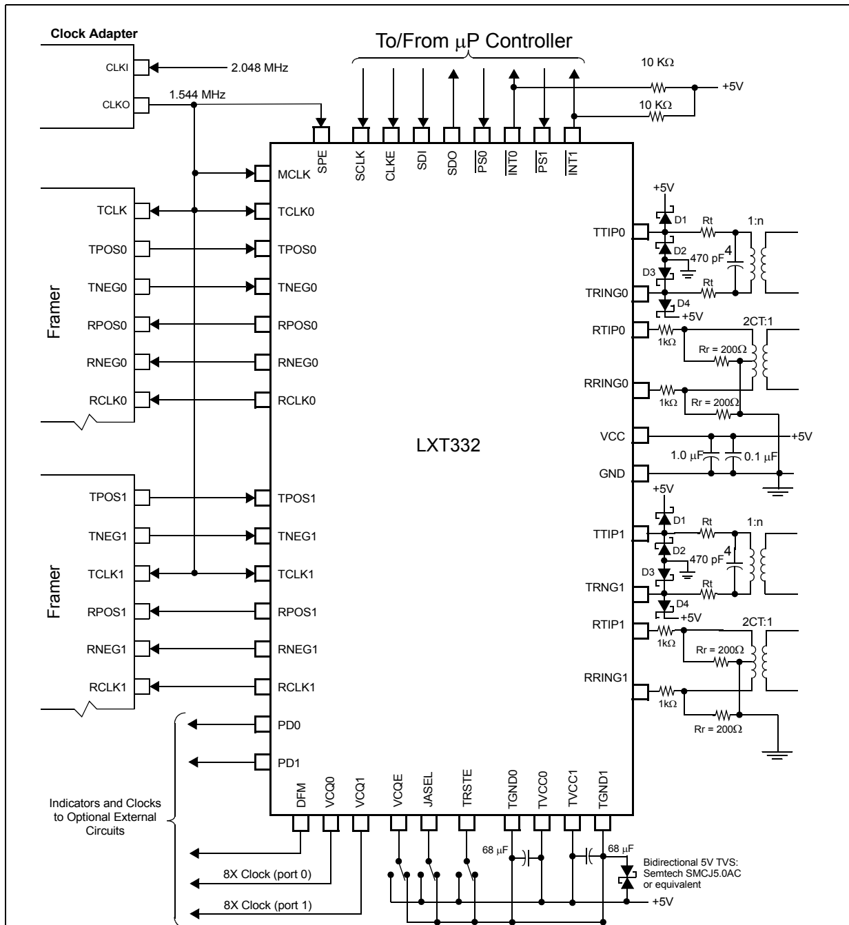
Figure 14 Typical T1 Application (Host Control Mode, Bipolar I/O)
