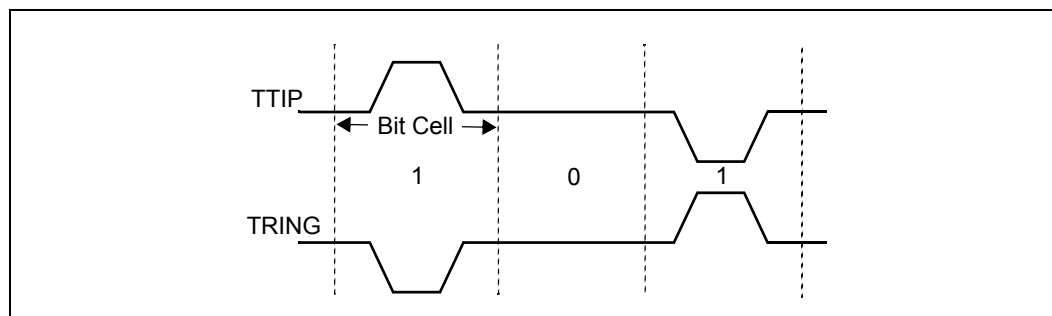
Figure 4 50% AMI Coding
