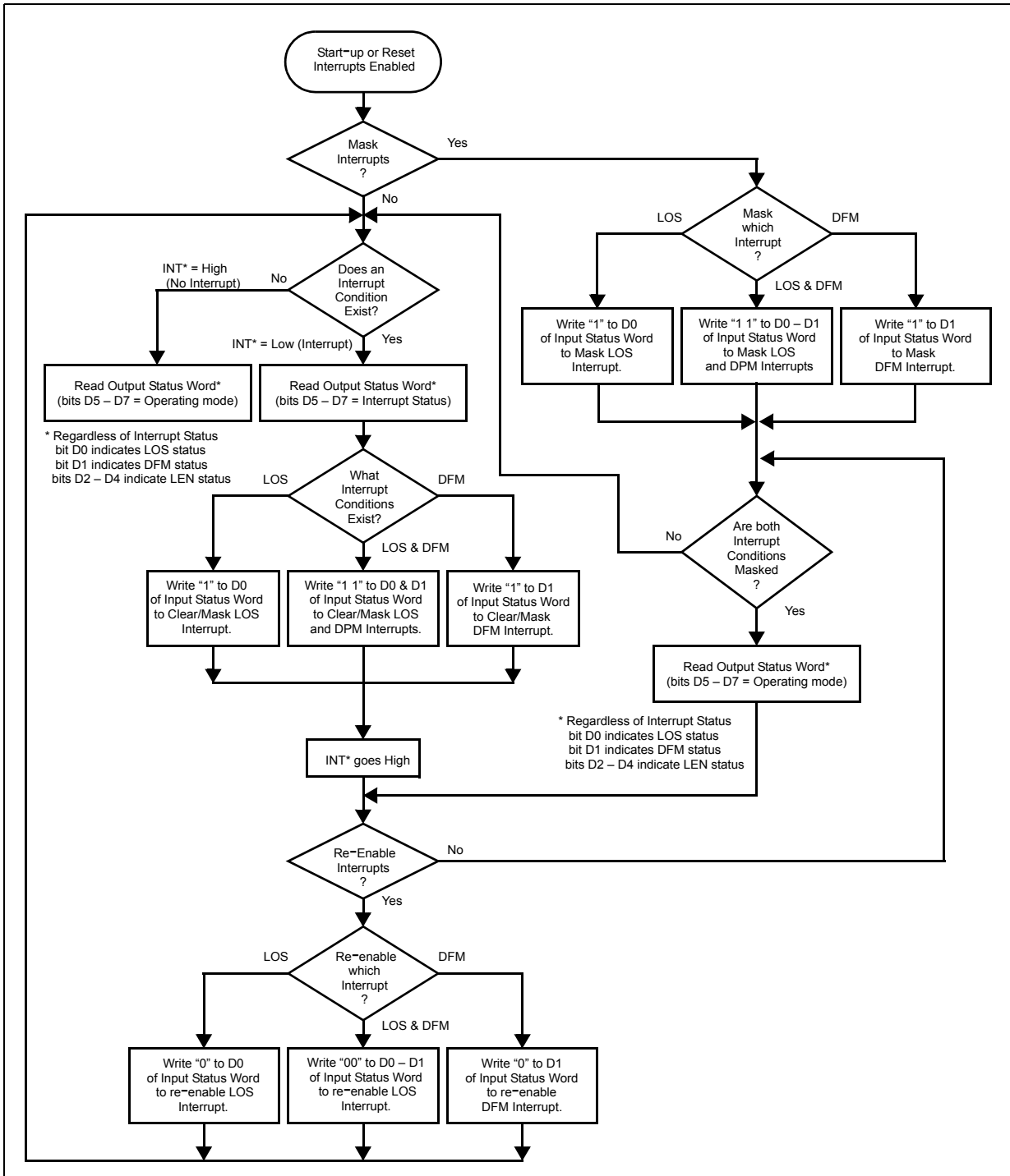
Figure 7 Interrupt Handling
