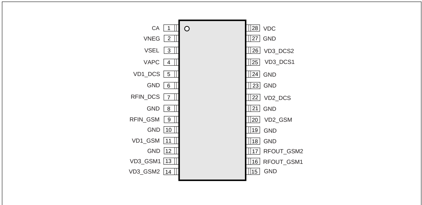
Figure 3. Pin configuration.
