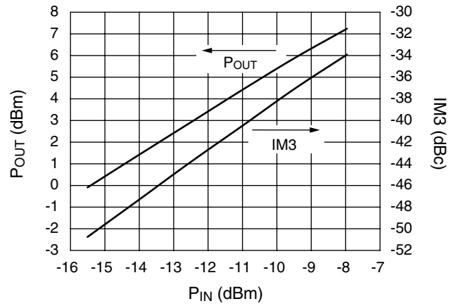
Output Power and Relative Third-Order Intermodulation Products F = 28 GHz, V DS = 6 V
