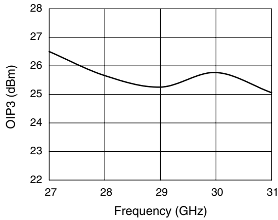
Two-Tone Output Third-Order Intercept @ V DS = 6 V
