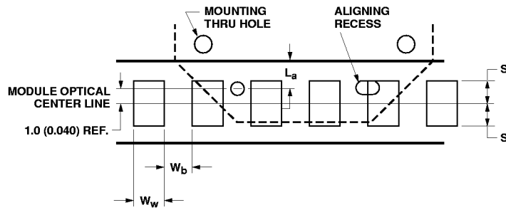
Figure 1. Codestrip Design.
