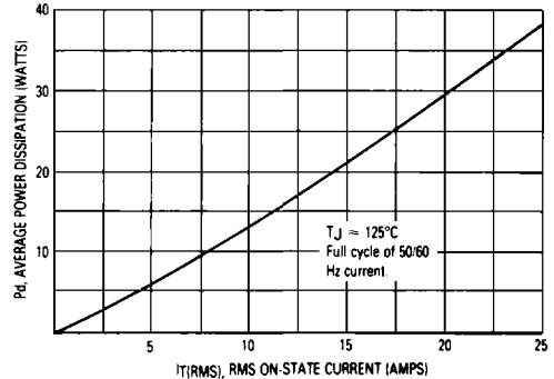
FIGURE 3 — ON-STATE POWER DISSIPATION
