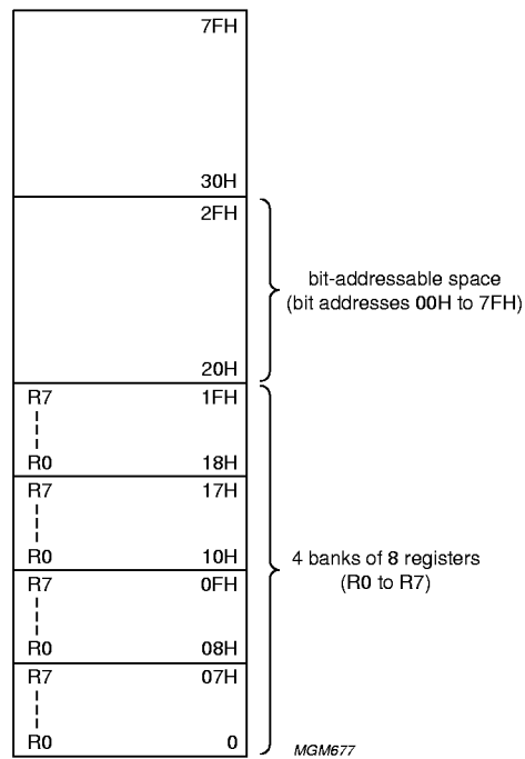
Fig.9 Lower 128 bytes of internal RAM.
