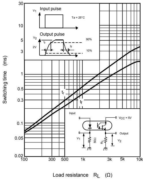
Switching Characteristics(non Saturated Operation) (typ.)
