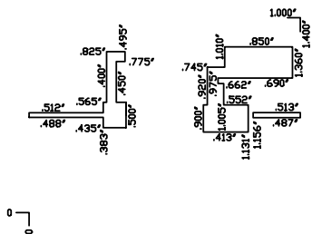
CIRCUIT DIMENSIONS
