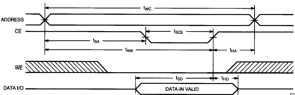
Write Cycle No. 2 ( \overline{CE} Controlled) [8, 13, 14]
