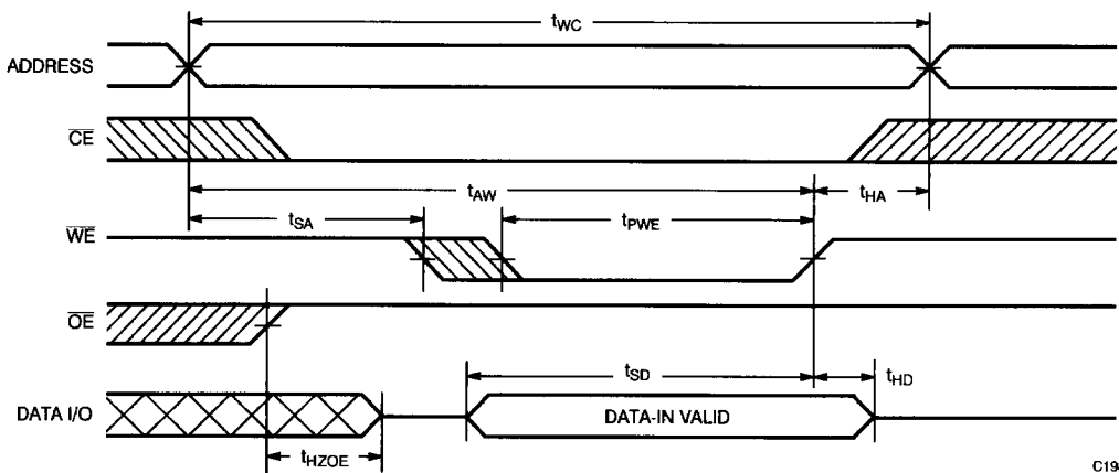
Write Cycle No. 1 ( \overline{WE} Controlled) [8, 13, 14]
