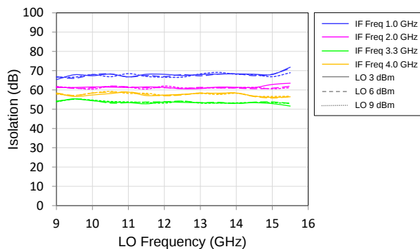
LSB IF-to-RF Isolation vs. LO Freq vs. IF and LO Power State: Max Gain
