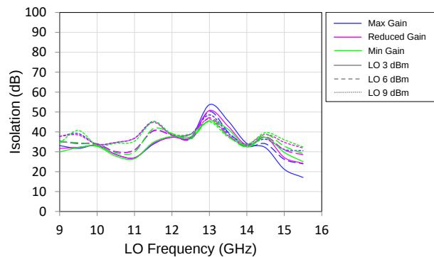
LSB LO-to-IF Isolation vs. LO Freq vs. LO Power and State
