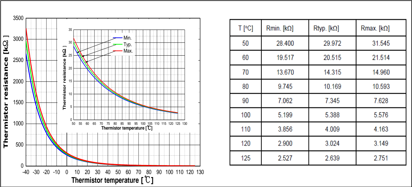
Figure 6 Thermistor resistance – temperature curve and table (For more information, please refer to the application note ‘AN2020-41 CIPOS™ Maxi application note’)
