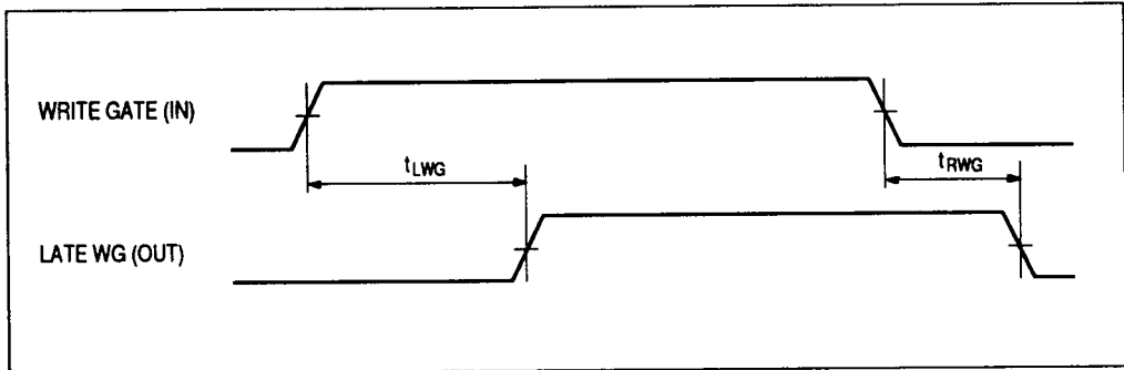
Fig 10 Late Write Gate
