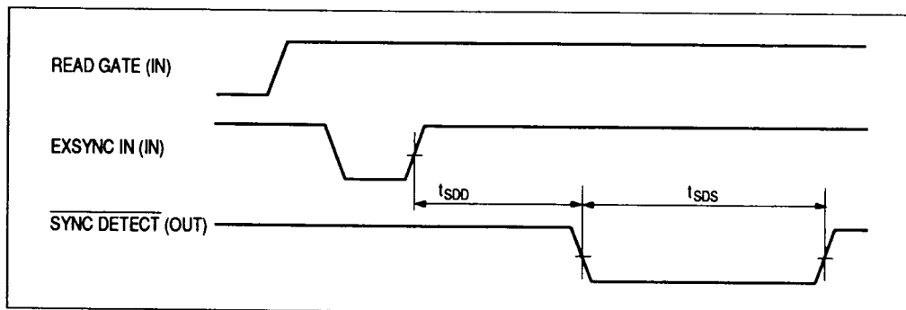
Figure 14 SYNC DETECT Output (Soft-sector Mode)
