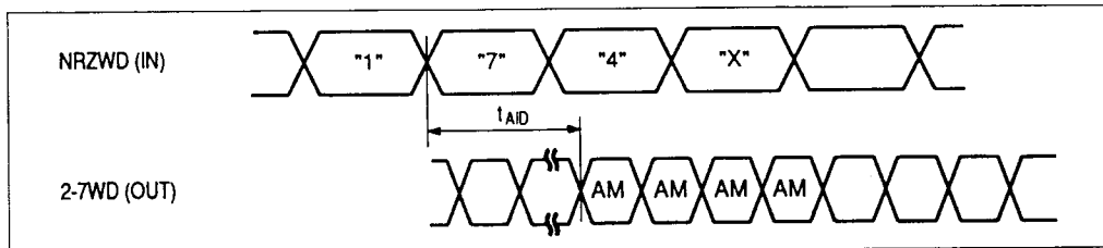
Figure 16 Address Mark Write (7-2 Illegal)
