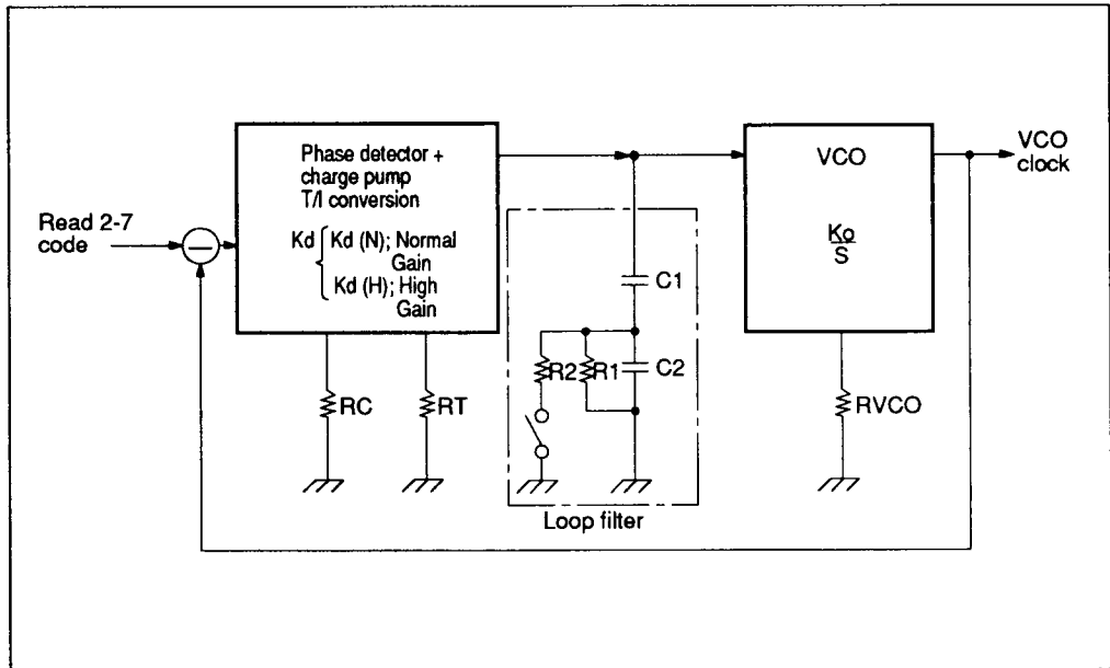
PLL Block Diagram
