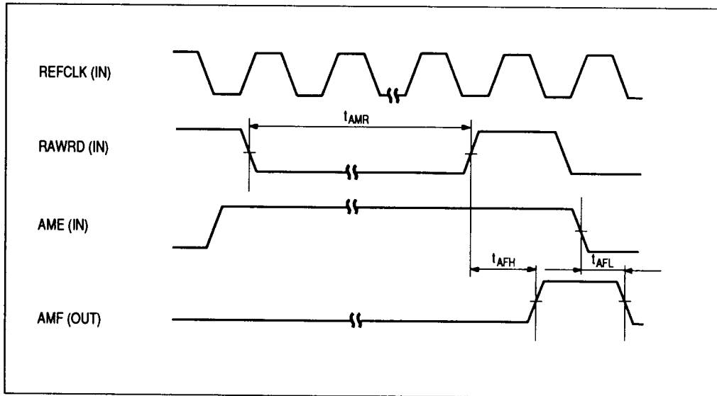
Figure 12 Address Mark Detection (DC Erase)
