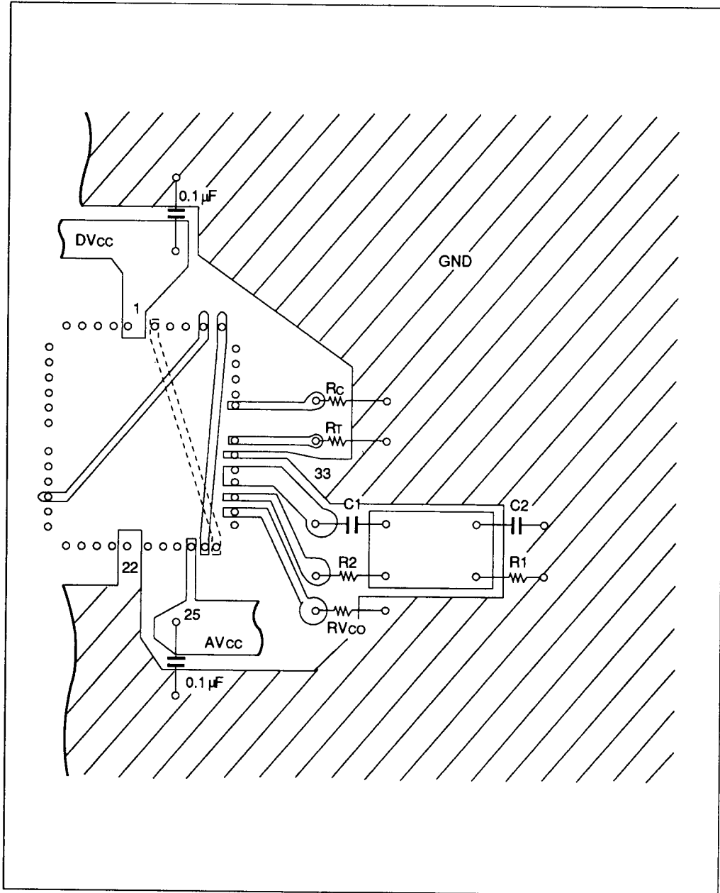
Figure 20 Recommend Print Pattern (Around the parts-connected pins)
