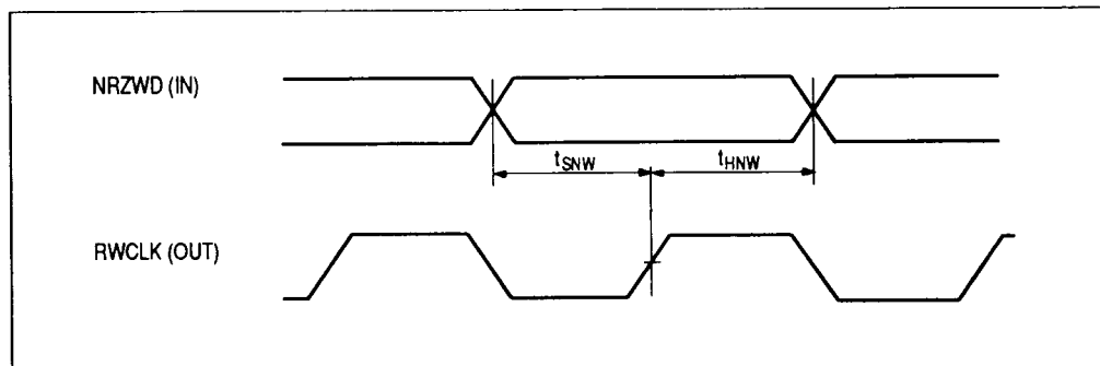
Figure 4 NRZ READ DATA Output
