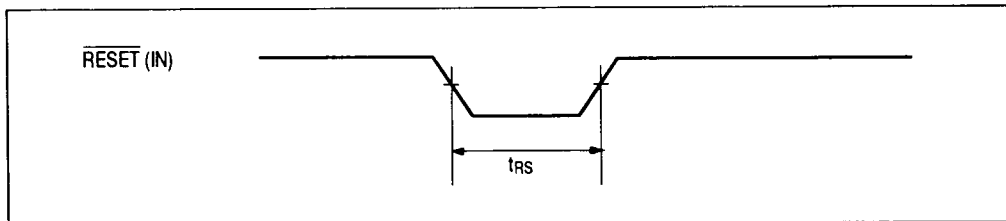
Figure 3 \overline{\text{RESET}} Input
