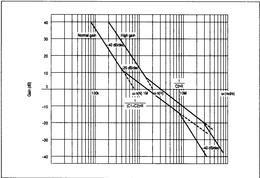
Figure 2 Bode Diagram Example when Maximum Transfer Rate is 15 Mbps
