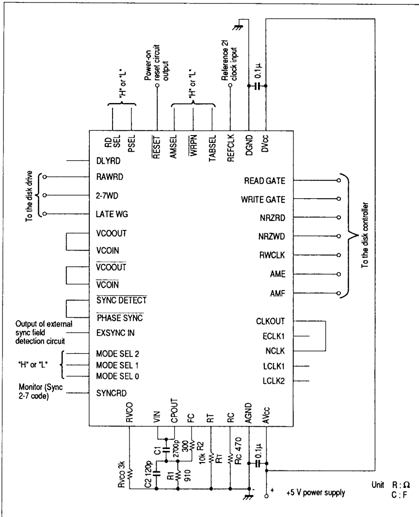
Figure 19 External Circuit Connection Example (15 Mbps)
