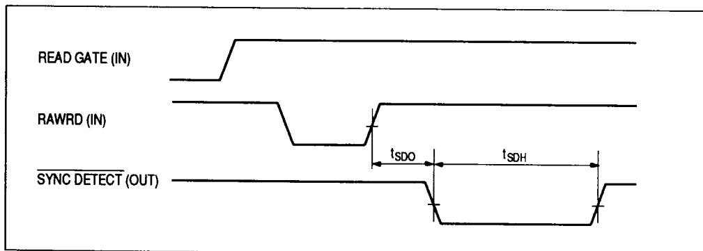
Figure 13 SYNC DETECT Output (Hard-sector Mode)
