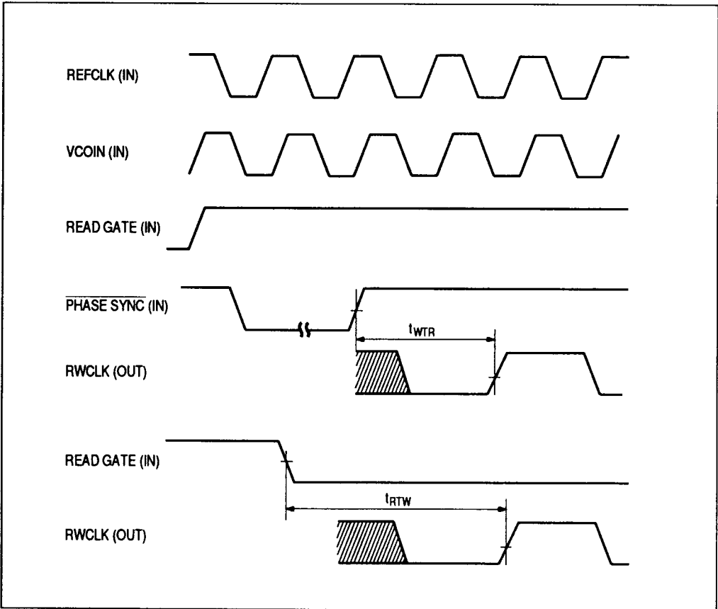
Figure 7 READ WRITE CLOCK
