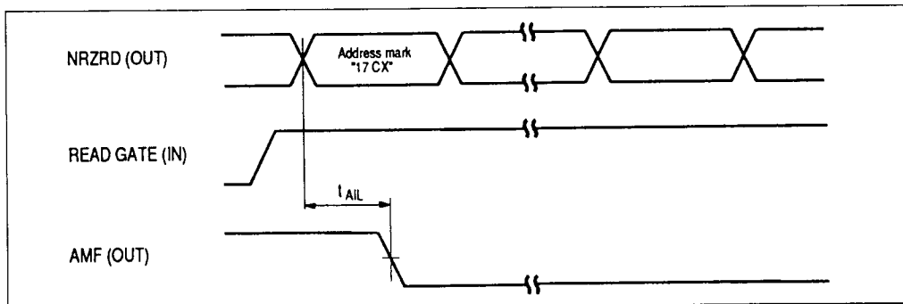
Figure 17 Address Mark Detection (7-2 Illegal)
