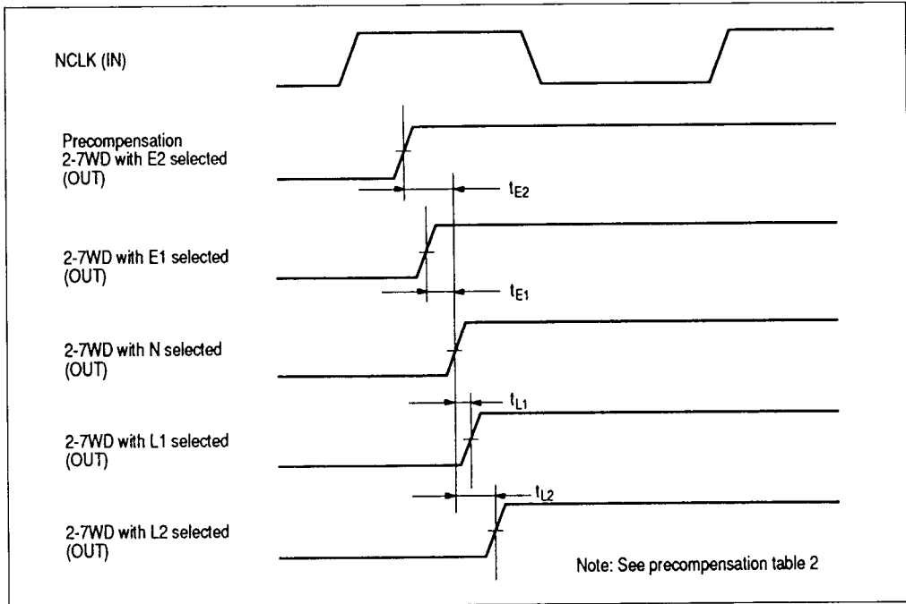
Figure 15 Write Precompensation in Internal Gate Delay Mode
