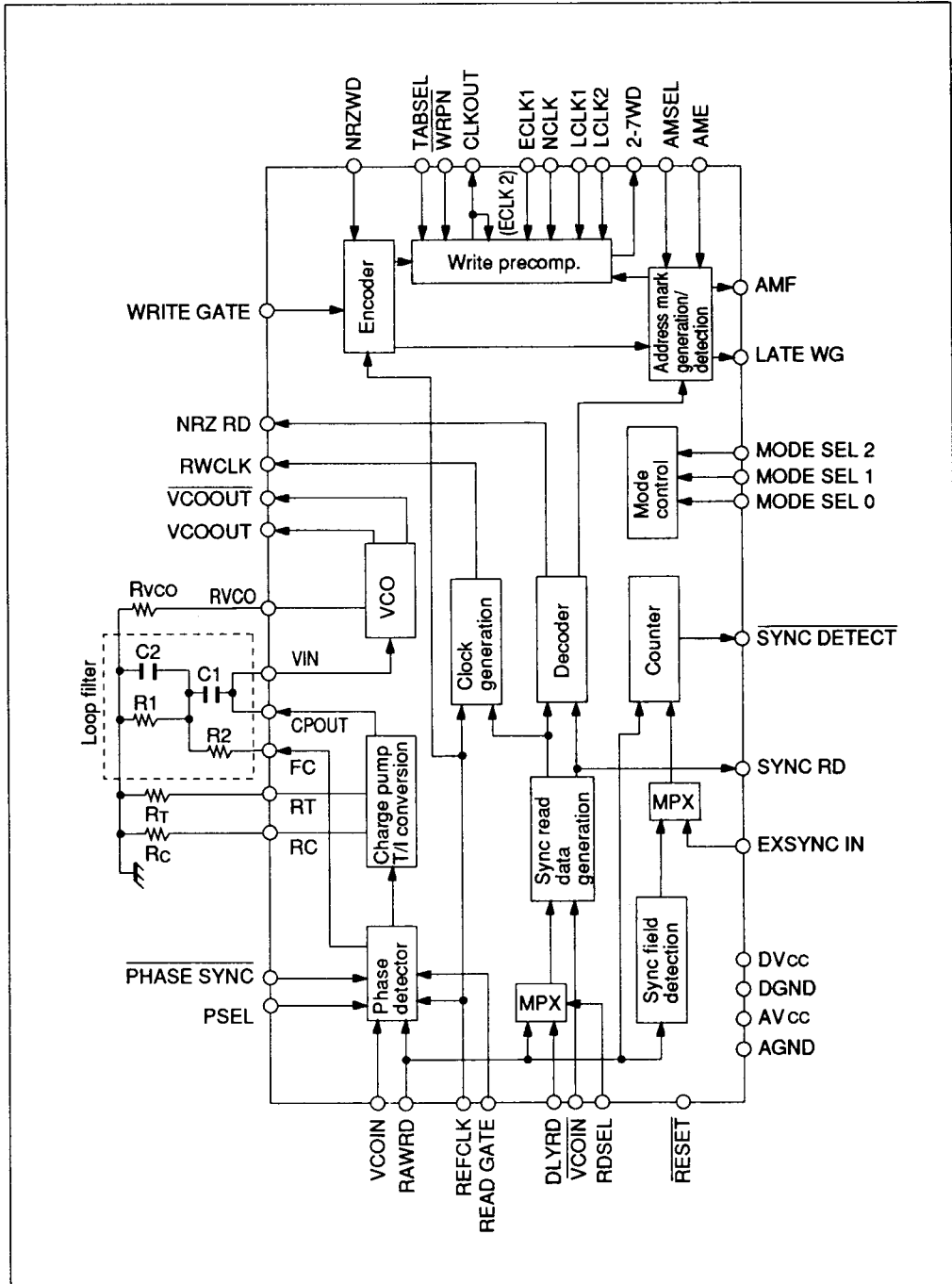
Block Diagram
