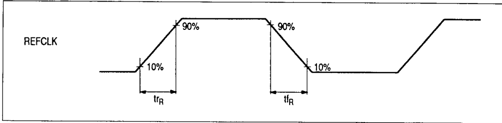
Figure 18 Reference Clock Rise and Fall Time
