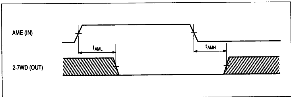
Figure 11 Address Mark Write (DC Erase)
