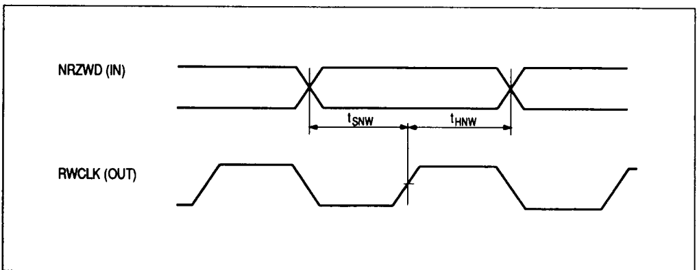
Figure 8 NRZ WRITE DATA Input
