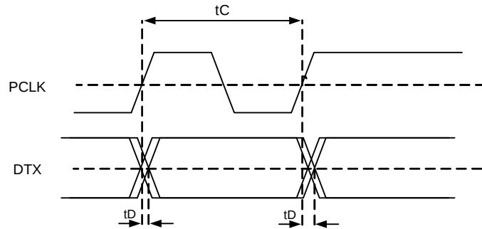
Figure 40: TDM Interface Input Delay AC Timing Diagram
