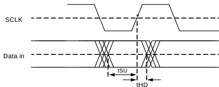
Figure 26: SPI (Master Mode) Normal Input AC Timing Diagram
