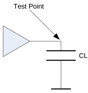
Figure 32: Device Bus Interface Test Circuit
