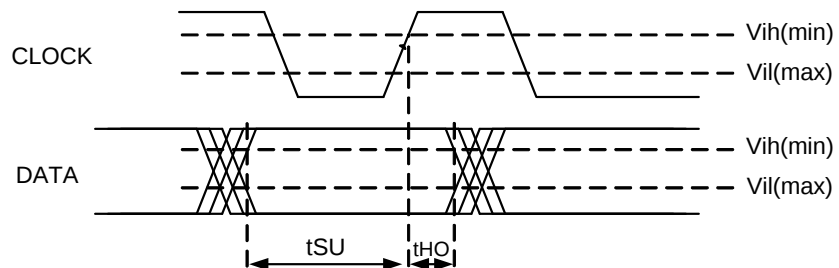
Figure 34: Device Bus Interface Input AC Timing Diagram
