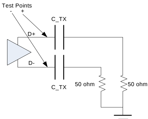
Figure 41: PCI Express Interface Test Circuit
