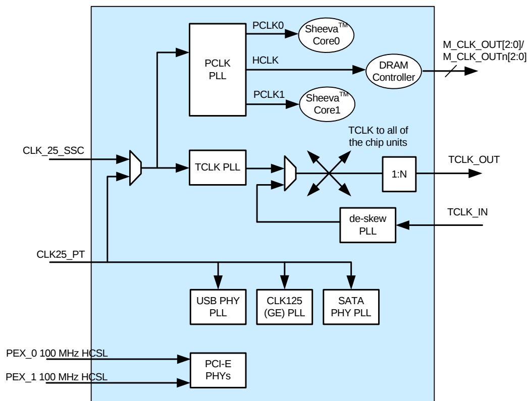
Figure 3: MV78200 Clocks
