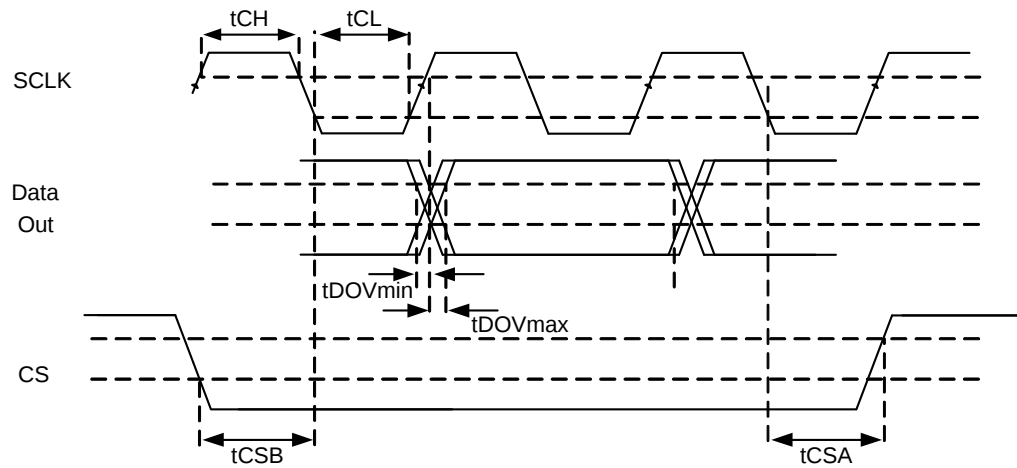
Figure 27: SPI (Master Mode) Opposite Output AC Timing Diagram
