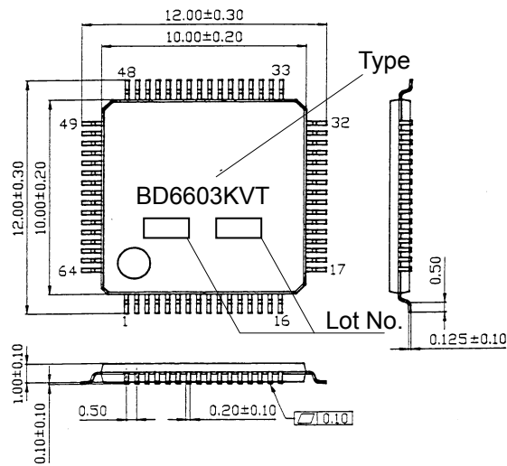
OPackage outlines
