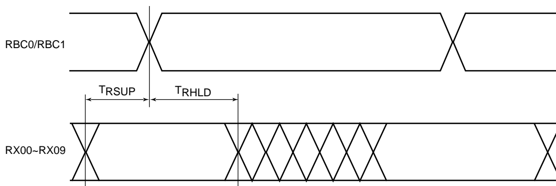
Figure 5: Receiver Timing 1
