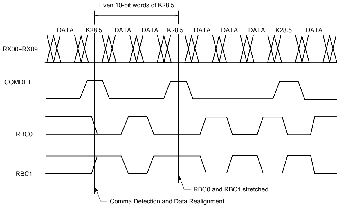
Figure 9: Synchronization Timing 3
