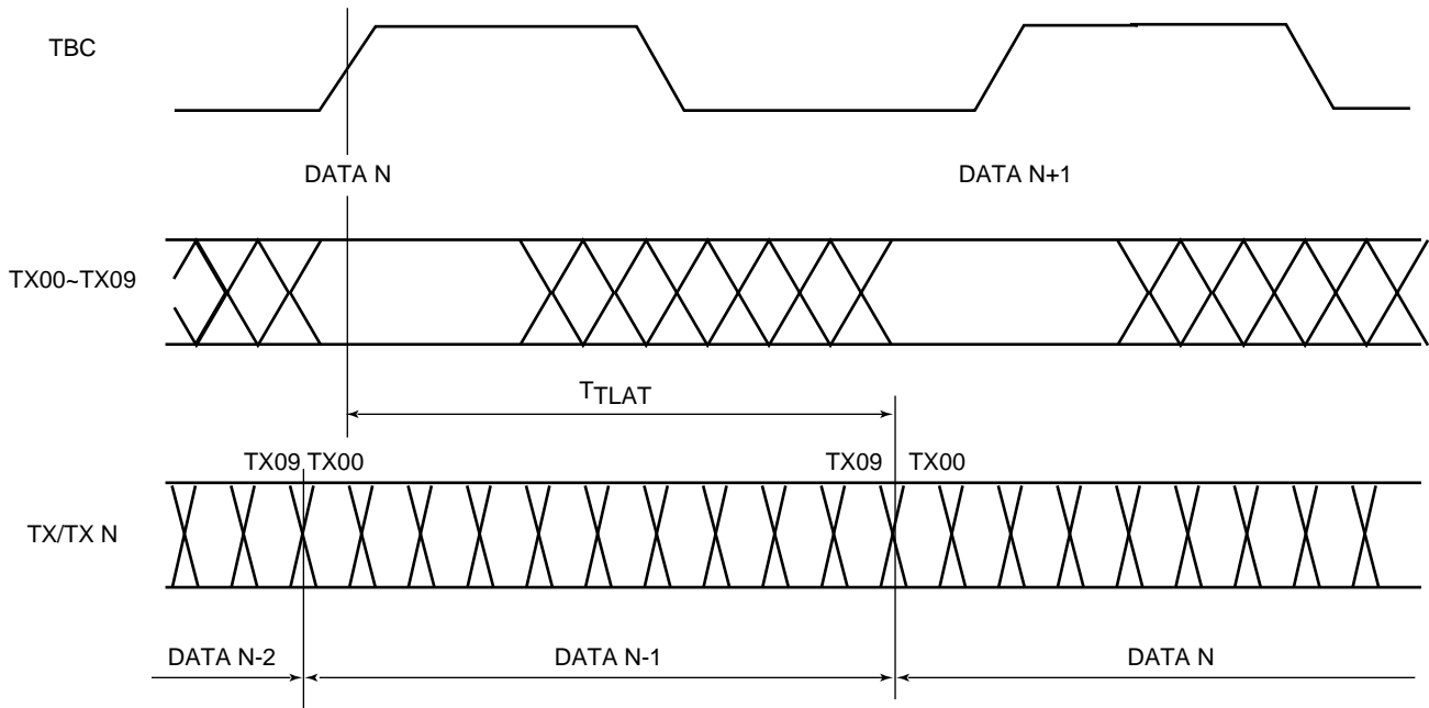
Figure 4: Transmitter Timing 2
