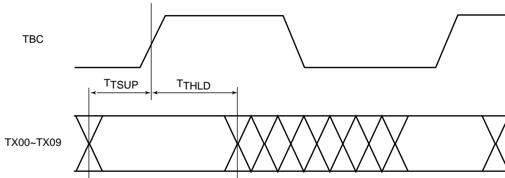
Figure 3: Transmitter Timing 1
