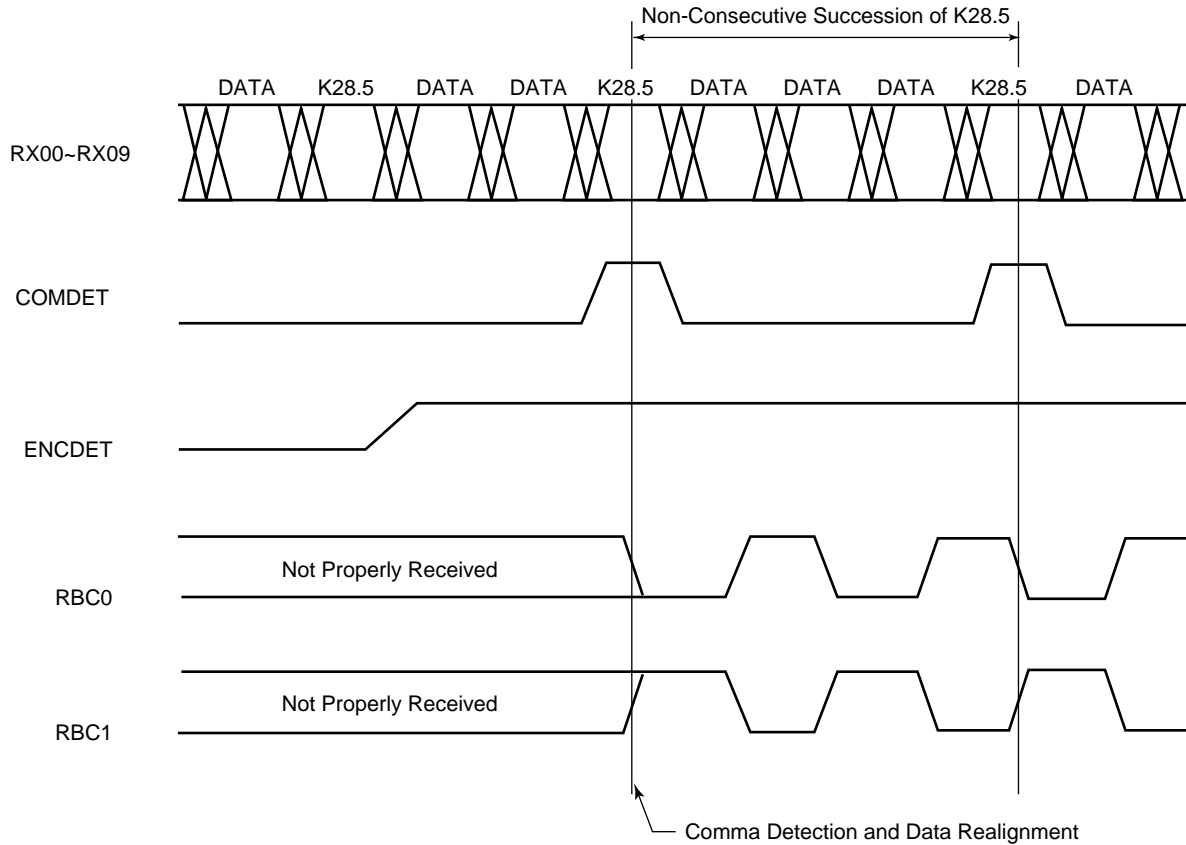
Figure 7: Synchronization Timing 1
