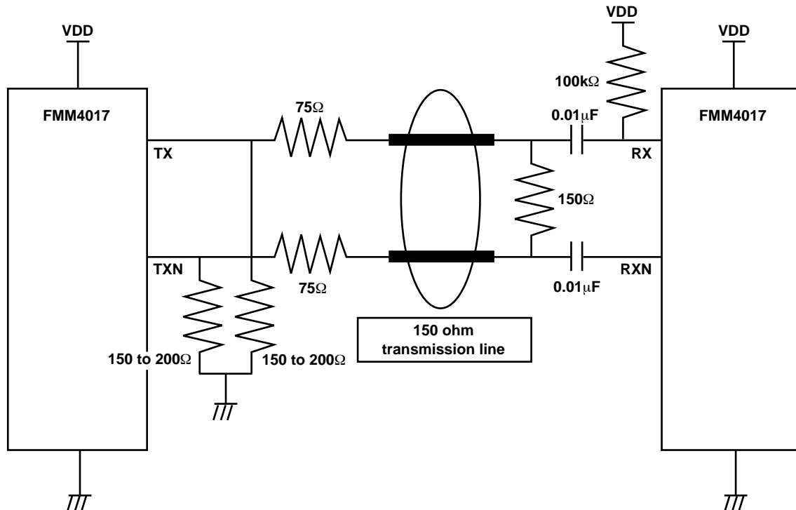
Figure 10: Termination Circuit for PECL Output
