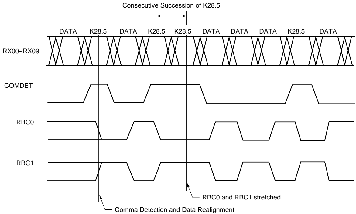
Figure 8: Synchronization Timing 2
