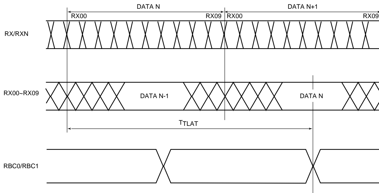
Figure 6: Receiver Timing 2
