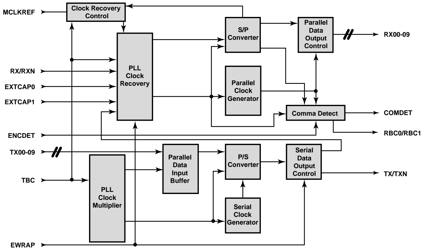
Figure 1: Functional Block Diagram of FMM4017KA/KB
