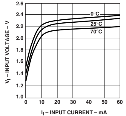
Figure 3. Typical Input Characteristics.
