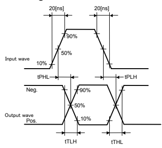
Switching characteristics
