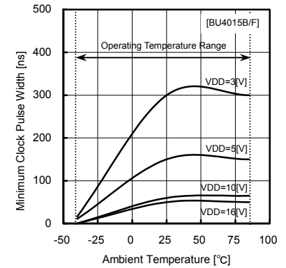
Fig.9 Minimum CLK pulse width
