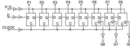
Block diagram
