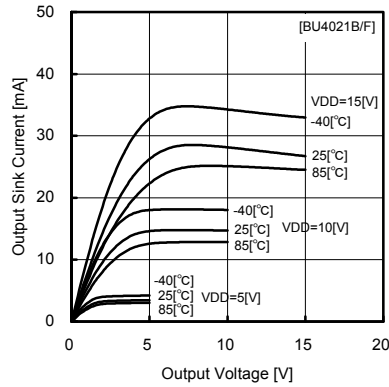
Fig. 12 Output sink current - voltage
