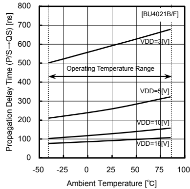
Fig. 15 Propagation delay tPLH P/S -> QS
