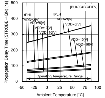
Fig.26 Propagation delay STROBE -> QN
