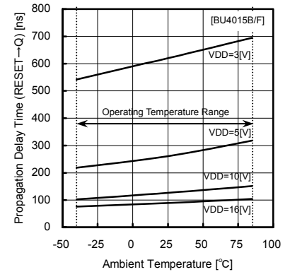
Fig.6 Propagation delay tPHL RESET→Q
