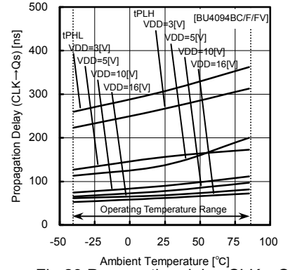
Fig.23 Propagation delay CLK -> QS
