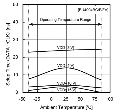
Fig.29 Set up time tsu DATA -> CLK
