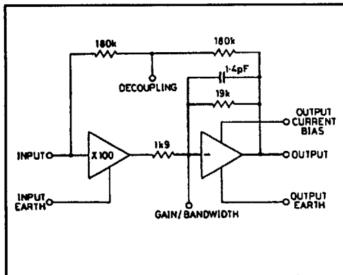
Fig.1 Circuit diagram
