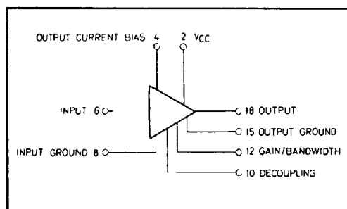
Fig.3 Pinning configuration - ZN460AM
