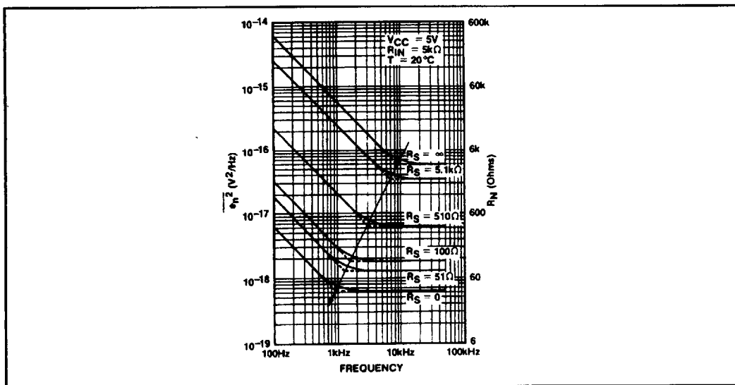
Fig.13 Noise voltage
