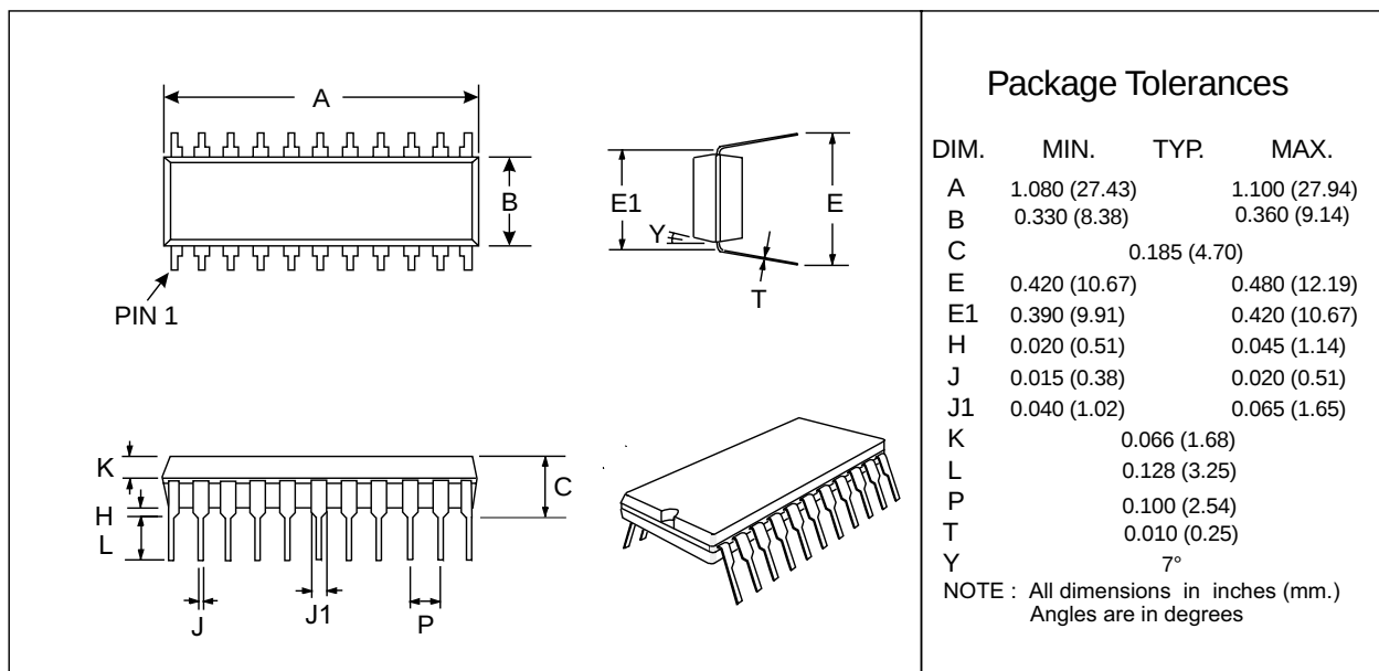
Figure 17: 22-pin PDIP (P6) Mechanical Outline: Order as part no. CMX629AP6
