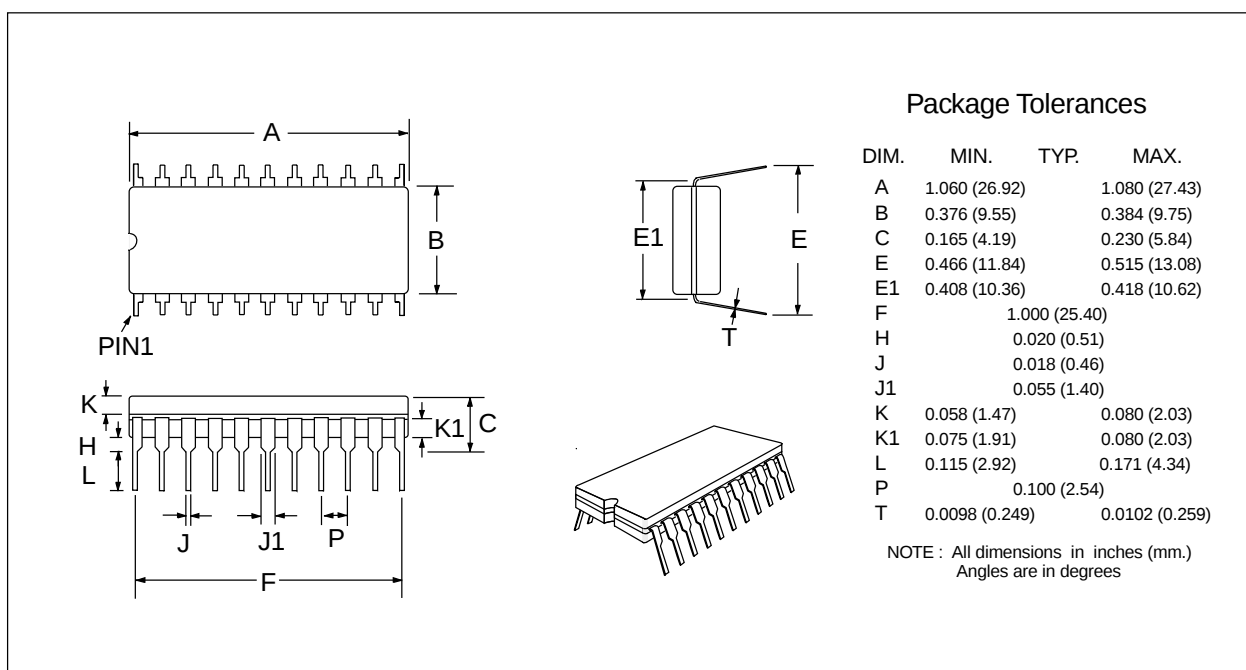
Figure 18: 22-pin Cerdip (J3) Mechanical Outline: Order as part no. CMX629AJ3
