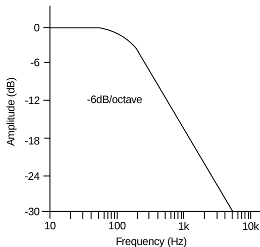
Figure 12: Principal Integrator Response
