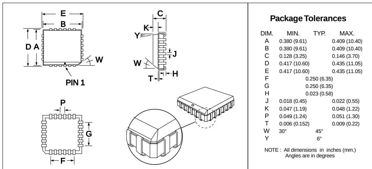
Figure 16: 24-pin PLCC (L2) Mechanical Outline: Order as part no. CMX629AL2
