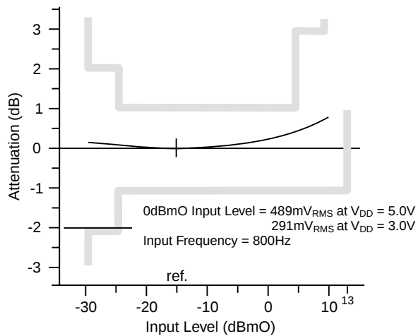
Figure 4: Gain vs. Input Level (16kbps)
