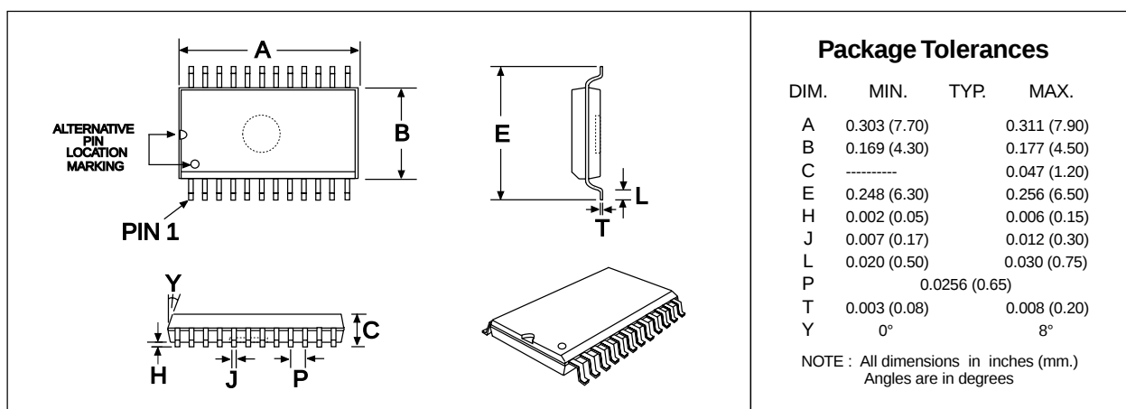
Figure 15: 24-pin TSSOP (E2) Mechanical Outline: Order as part no. CMX629AE2
