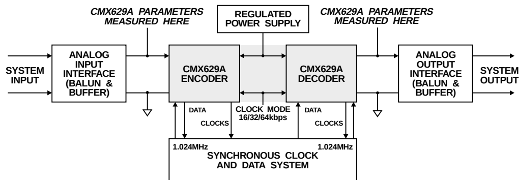
Figure 3: System Configuration using the CMX629A
