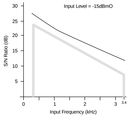
Figure 11: S/N vs. Input Frequency (32kbps)
