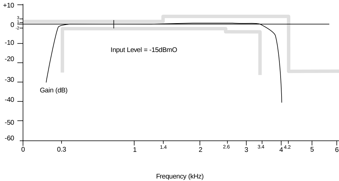
Figure 9: Attenuation Distortion vs. Frequency (32kbps)
