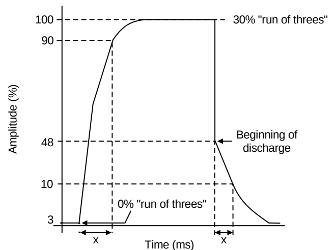
Figure 13: Compand Envelope
