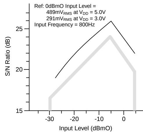
Figure 7: S/N vs. Input Level (32kbps)
