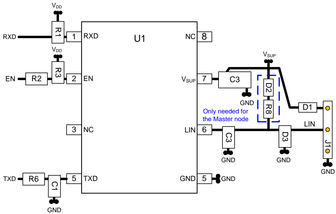
Figure 33. Layout Example
