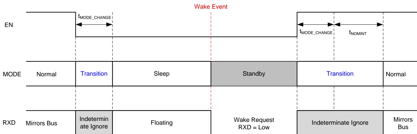
Figure 22. Mode Transitions
