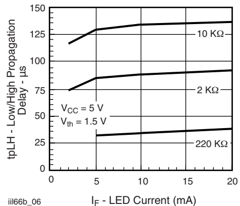
Fig. 8 - Low to High Propagation Delay vs. Collector Load Resistance and LED Current
