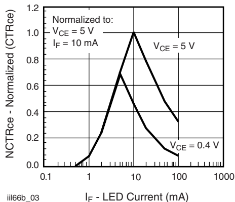
Fig. 5 - Normalized Non-Saturated and Saturated CTR_{CE} vs. LED Current
