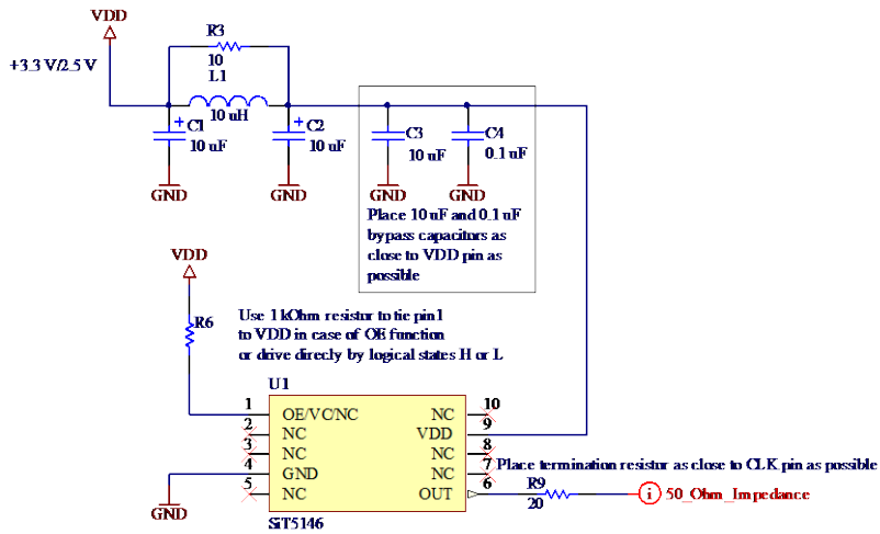
Figure 50. TCXO schematic example
