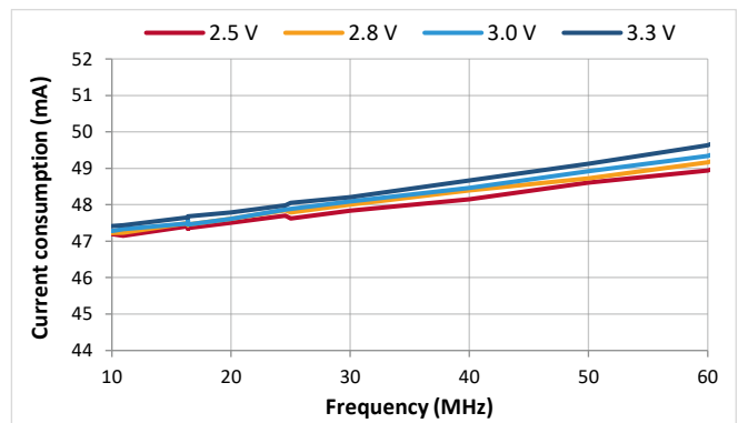
Figure 22. IDD VTCXO (LVCMOS)
