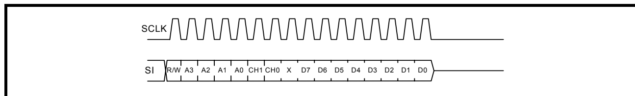
FIGURE 7. SPI WRITE
