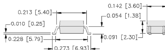
Package Style A (SMD)
