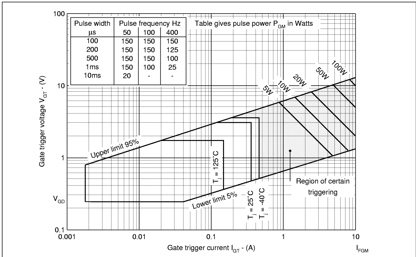
Fig.4 Gate characteristics
