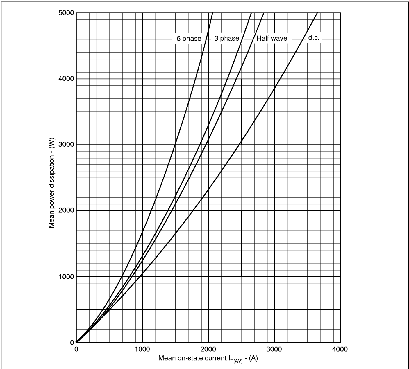
Fig.2 Dissipation curves
