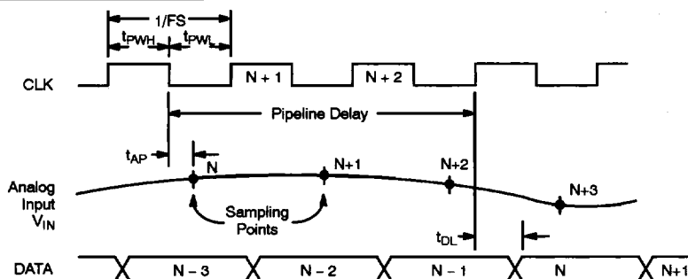
Figure 1. XRD66L92 Timing Diagram
