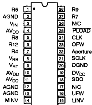
28 Pin PDIP (0.600")
