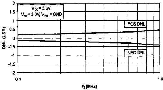
Graph 1. DNL vs. F_s
