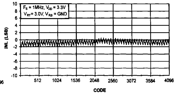
Graph 5. INL Error Plot
