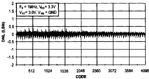
Graph 4. DNL Error Plot
