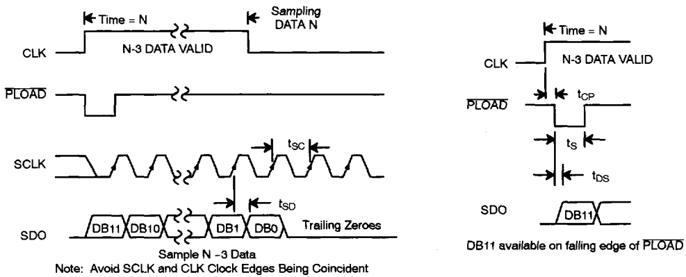
Figure 4. Serial Port Timing Chart PHASE = 1
