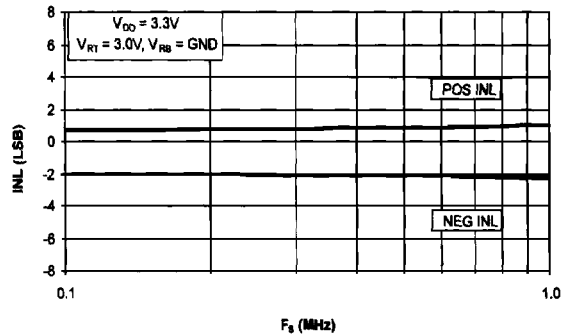
Graph 2. INL vs. F_s
