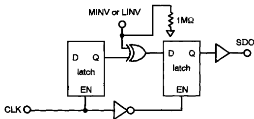
Figure 5. MINV, LINV Simplified Logic Circuit
