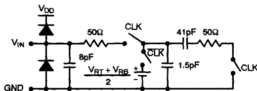
Figure 6. Equivalent Input Circuit
