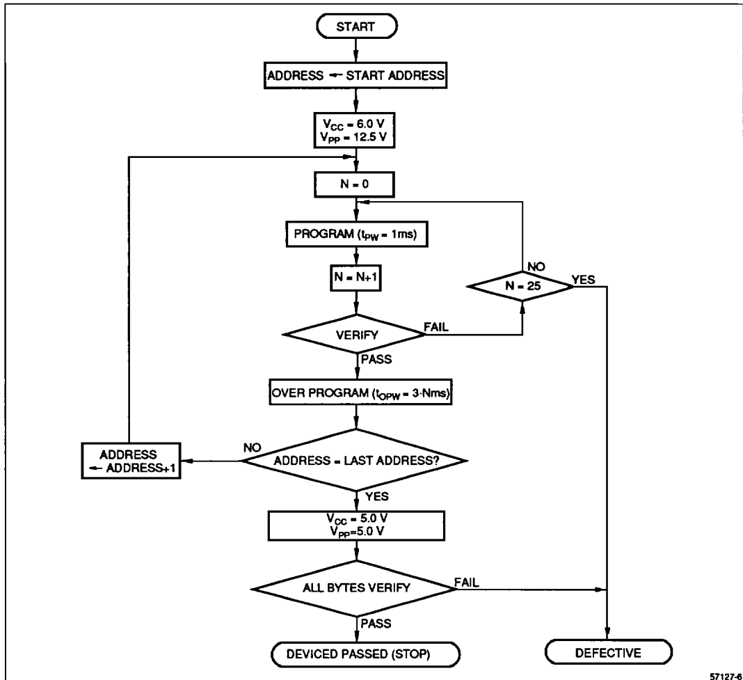
Figure 6. Programming Flowchart
