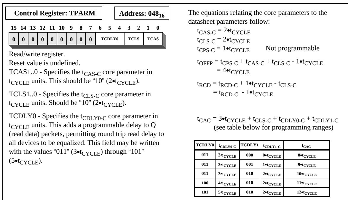
Figure 39: TPARM Register
