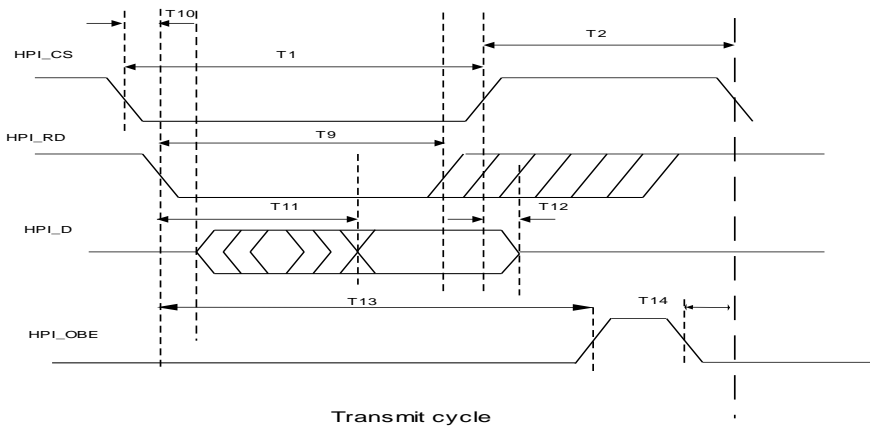
Transmit cycle
