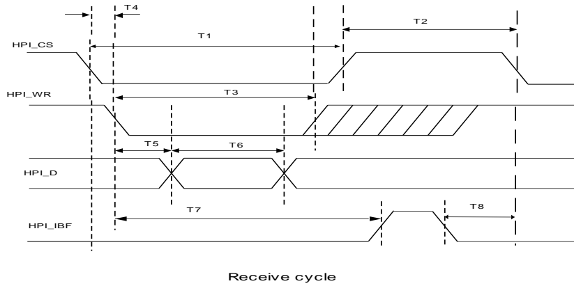
Receive cycle
