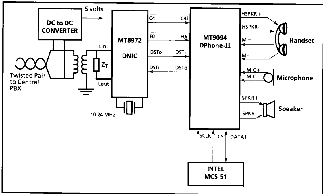
Figure 10 - Voice/Data Digital Telephone Set Circuit
