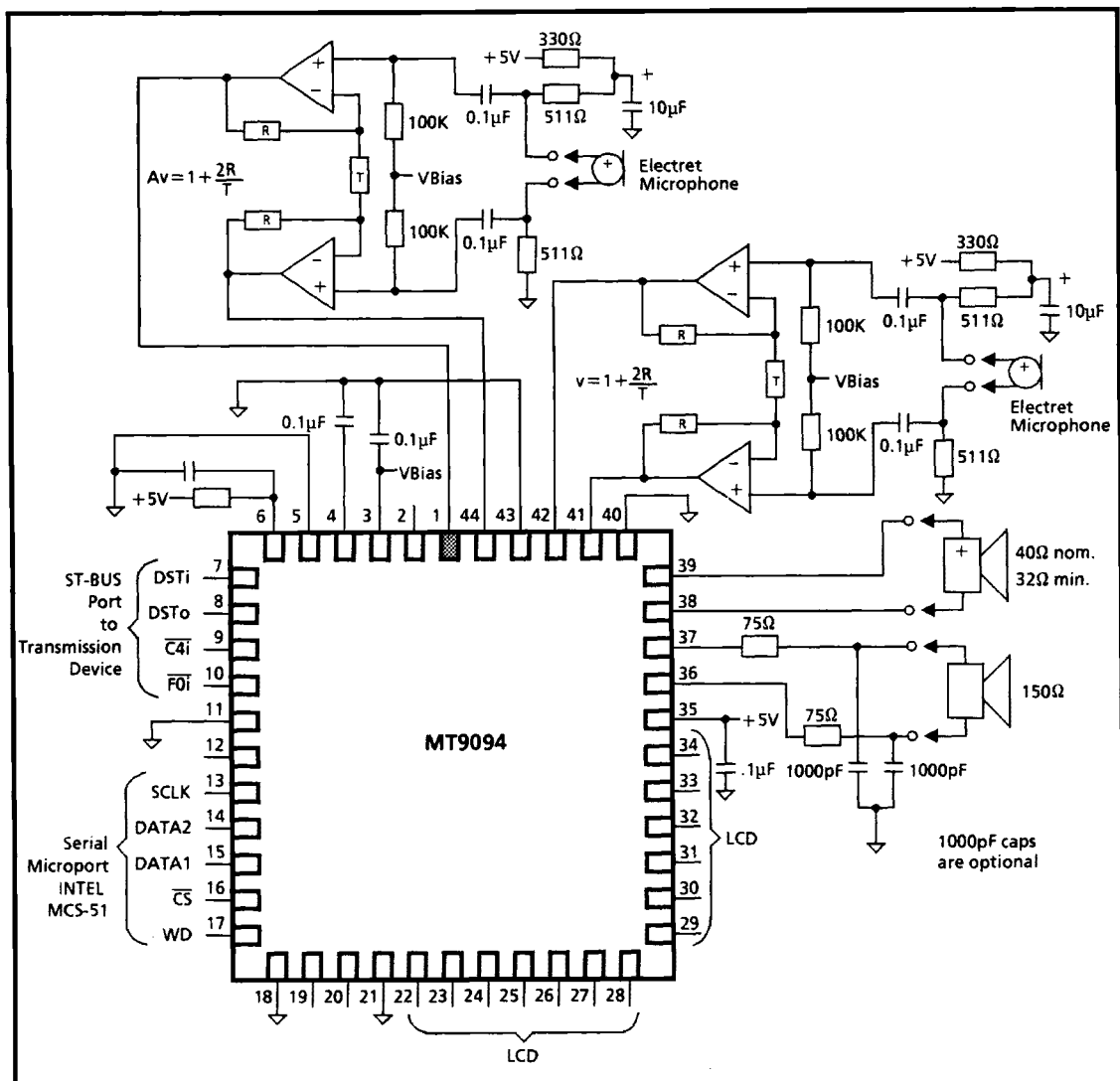
Figure 7 - Application Circuit - fully differential audio input
