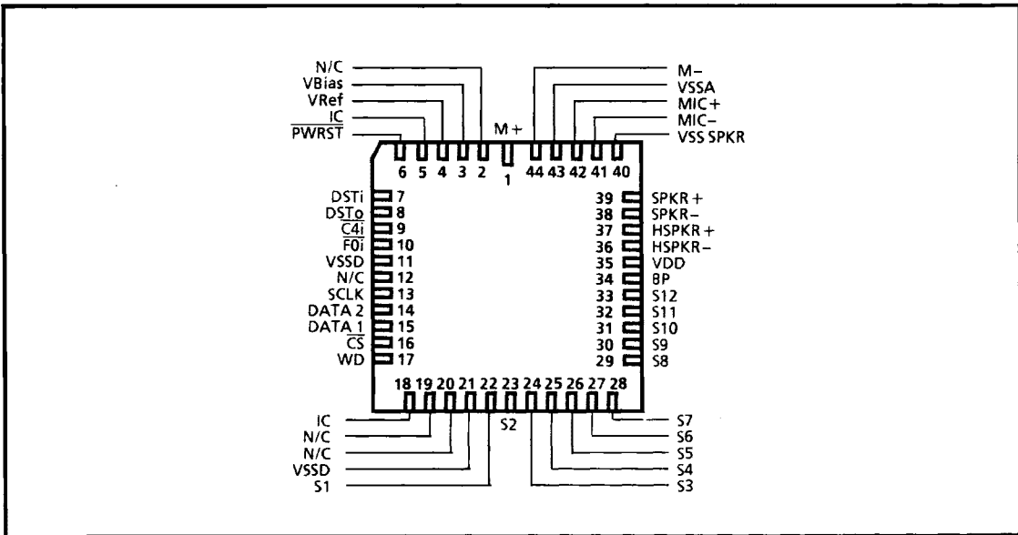
Figure 2 - Pin Connections
