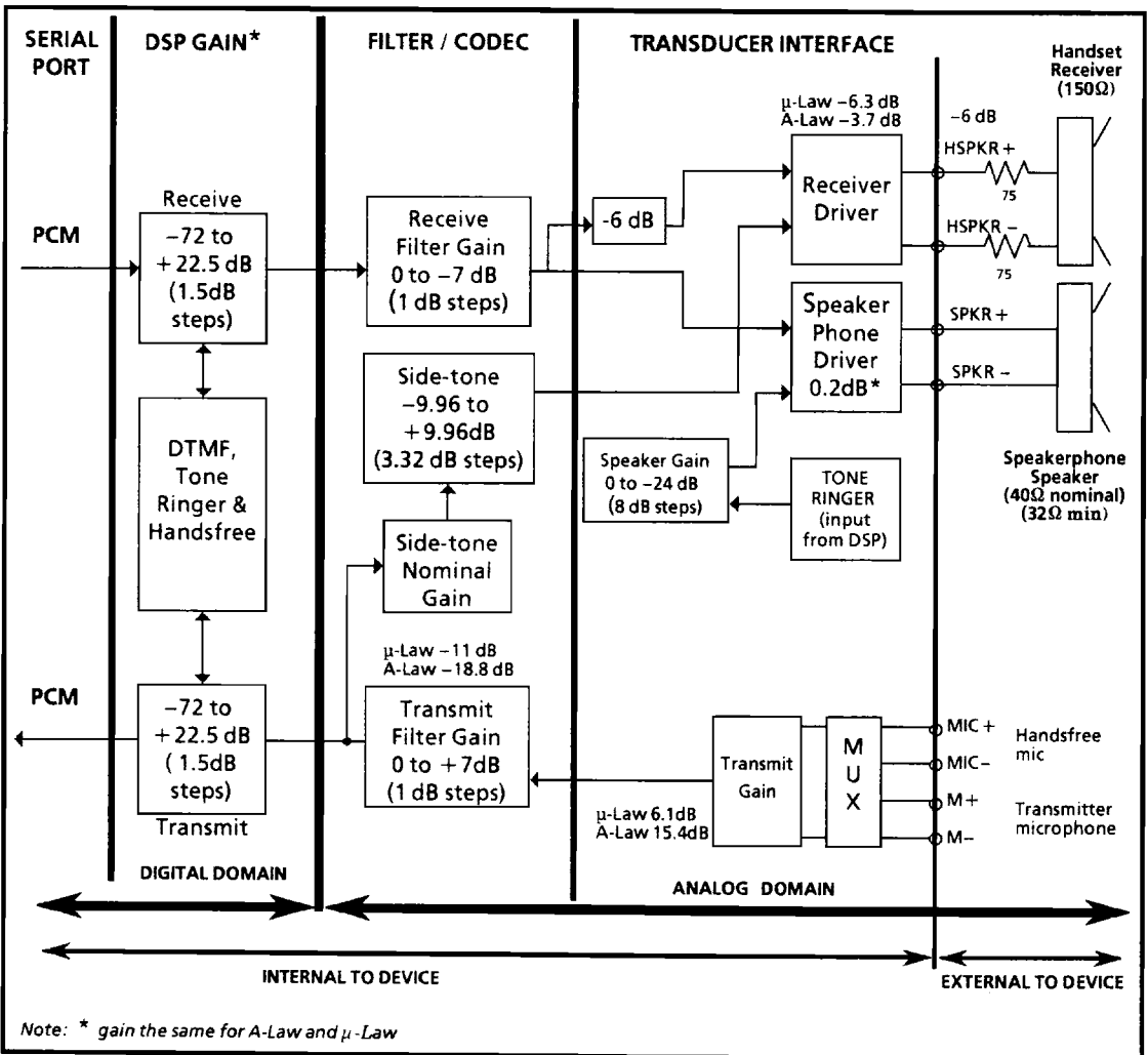
Figure 3 - Audio Gain Partitioning
