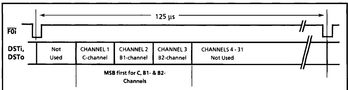
Figure 6 - ST-BUS Channel Assignment
