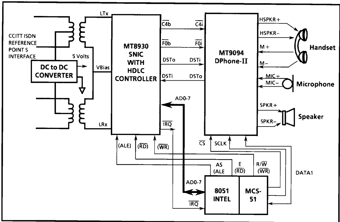
Figure 9 - CCITT ISDN Voice/Data Terminal Equipment - TE1
