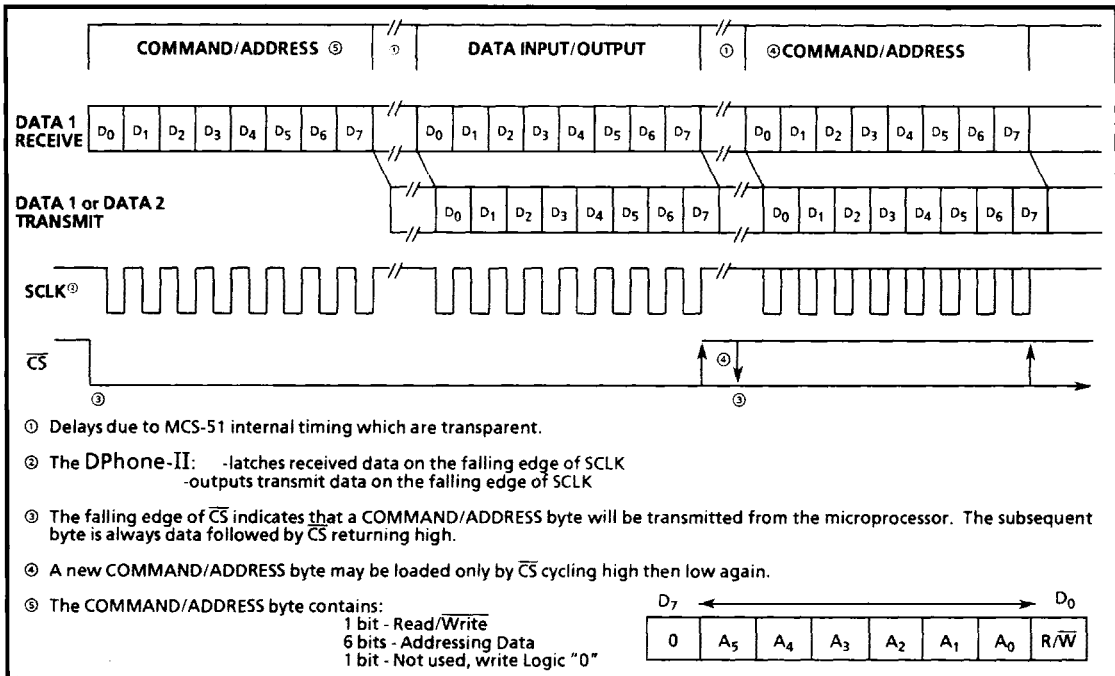
Figure 5 - Serial Port Relative Timing
