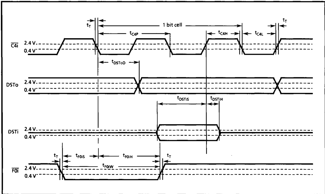
Figure 11 - ST-BUS Timing Diagram
