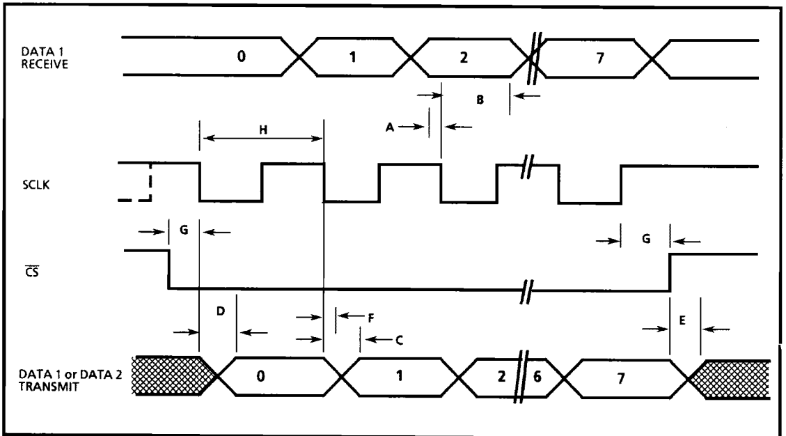
Figure 12 - Serial Microport Timing Diagram
