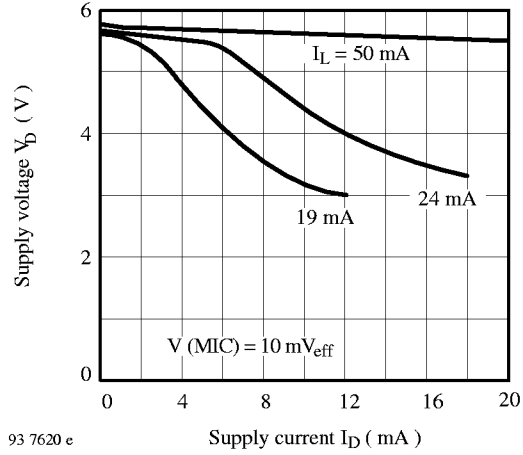
Figure 3. Supply voltage, V D
