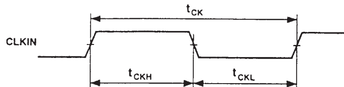
Figure 3. Clock
