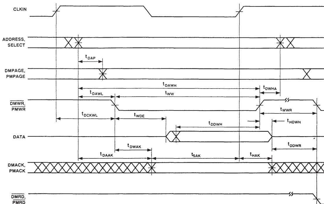
Figure 11. Memory Write
