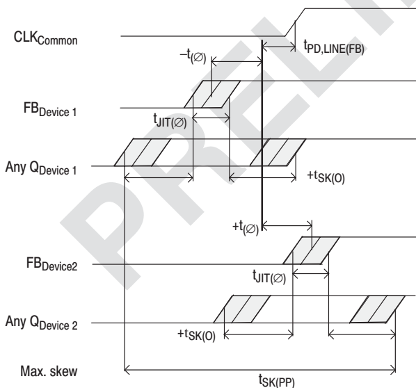
Figure 7. MPC9990 max. device-to-device skew
