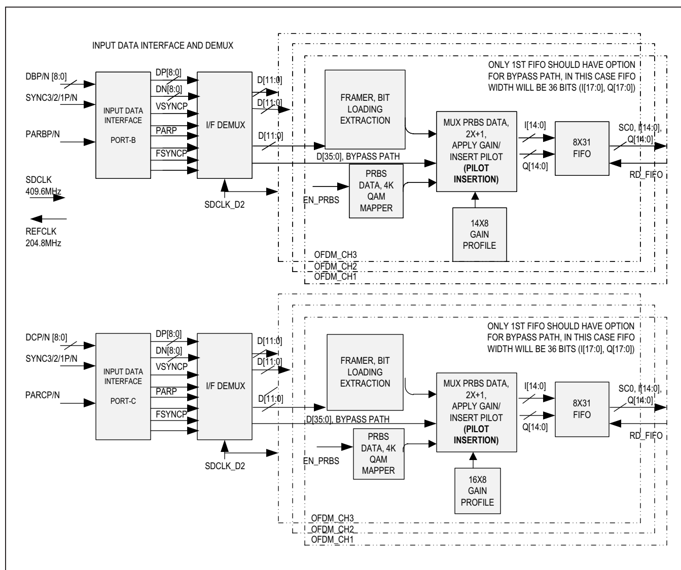
Figure 14. Input Data Interface Detailed Block Diagram
