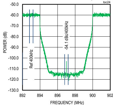
GAP SUBCARRIER POWER FOR MIXED 2OFDM + 24 SCQAM CF = 921MHz OFDM 192MHz 1024 QAM Ncp = 512, Nrp = 256 toc24
