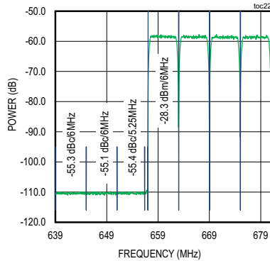
LOWER ACP FOR MIXED 2OFDM + 24SCQAM CF = 921MHz OFDM 192MHz 1024 QAM Ncp = 512, Nrp = 256 toc22
