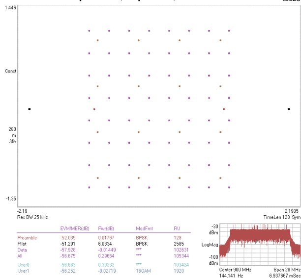
MER FOR 24MHz OFDM 64 QAM 25kHz SPACING Ncp = 1024, Nrp = 128, CF = 900MHz
