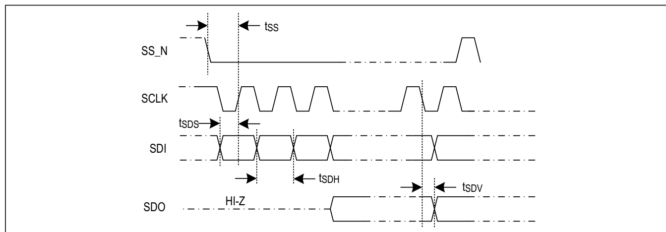
Figure 30. SPI Timing Diagram
