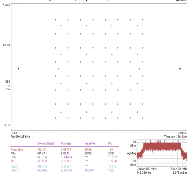
MER FOR 24MHz OFDM 64 QAM 25kHz SPACING Ncp = 1024, Nrp = 128, CF = 300MHz
