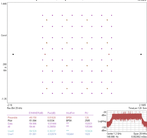
MER FOR 24MHz OFDM 64 QAM 25kHz SPACING Ncp = 1024, Nrp = 128, CF = 1200MHz
