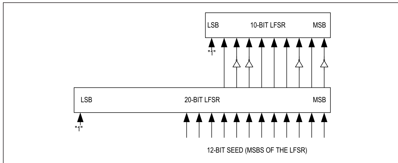
Figure 40. LFSR Seeds
