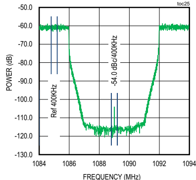
GAP SUBCARRIER POWER FOR MIXED 2OFDM + 24 SCQAM CF = 921MHz OFDM 192MHz 1024 QAM Ncp = 512, Nrp = 256 toc25
