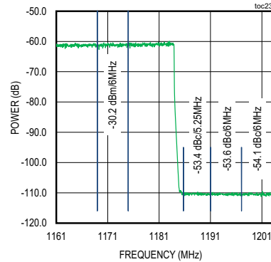
UPPER ACP FOR MIXED 2OFDM + 24 SCQAM CF = 921MHz OFDM 192MHz 1024 QAM Ncp = 512, Nrp = 256 toc23
