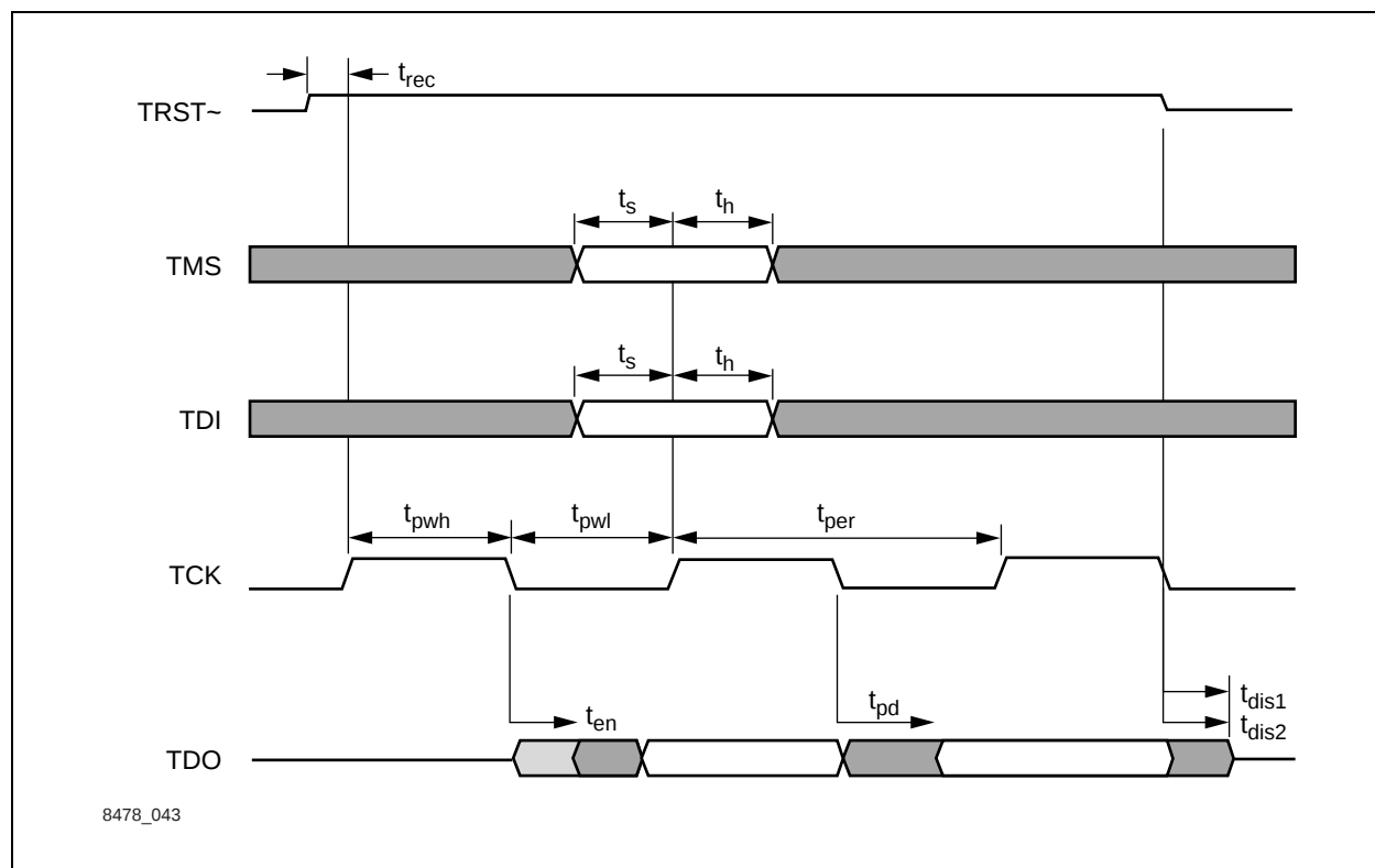
Figure A-1. JTAG Timing Diagram
