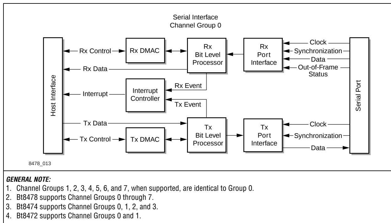
Figure 4-1. Serial Interface Functional Block Diagram, Channel Group 0
