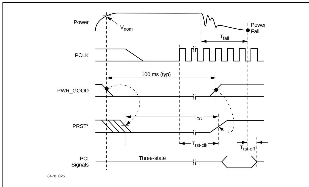
Figure 7-2. PCI Reset Timing
