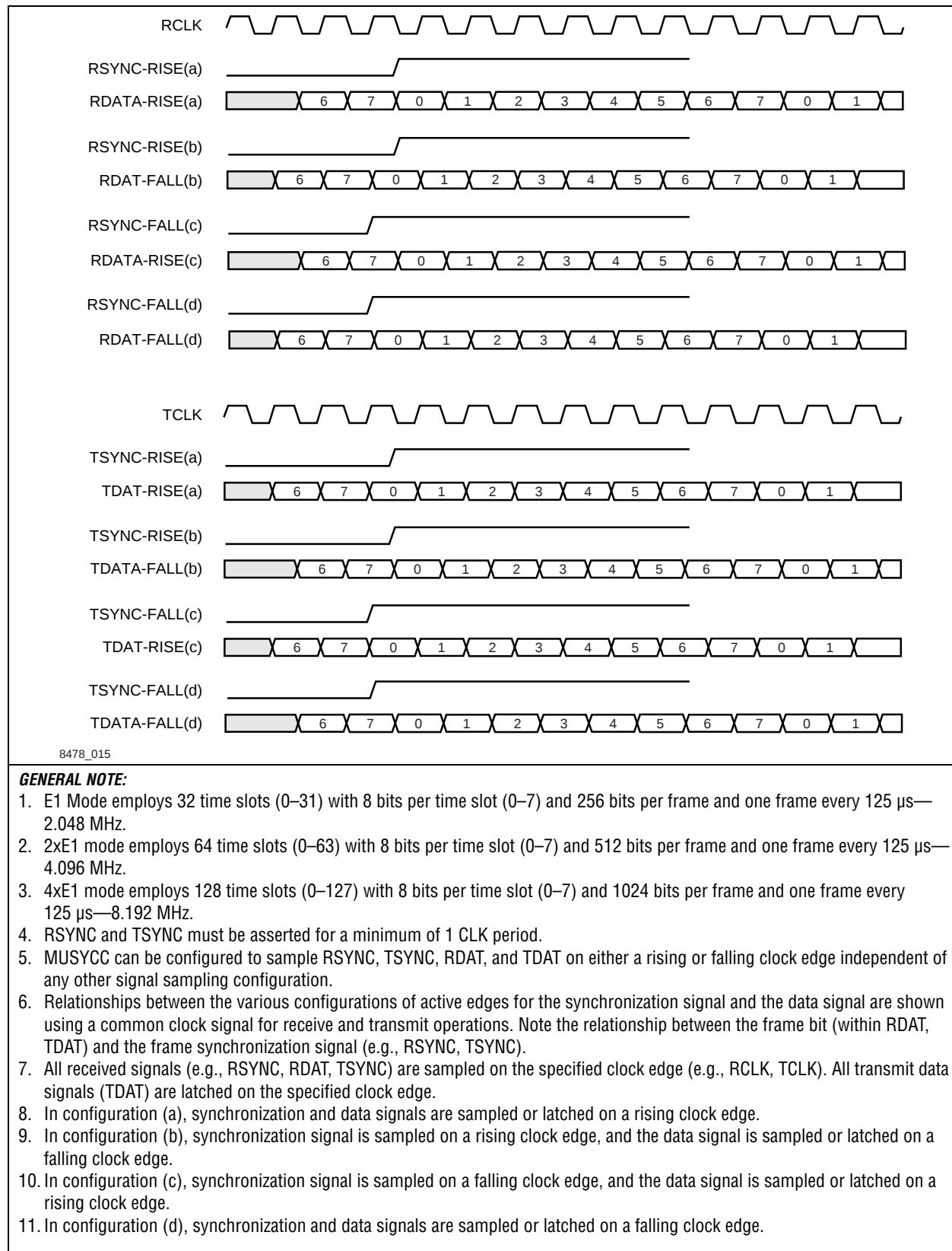
Figure 4-3. Transmit and Receive E1 (also 2xE1, 4xE1) Mode
