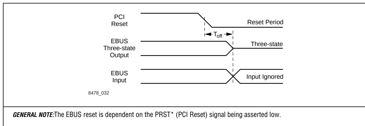
Figure 7-10. EBUS Reset Timing
