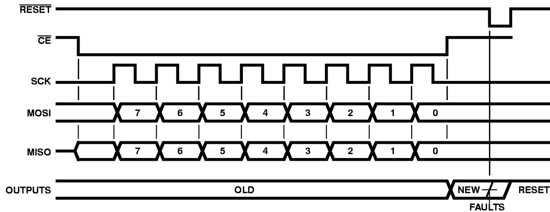
FIGURE 8. BYTE TIMING DIAGRAM WITH ASYNCHRONOUS RESET
