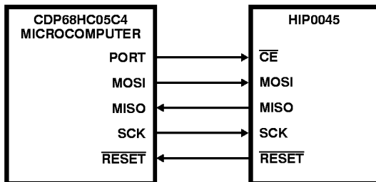
FIGURE 9. TYPICAL MICROCOMPUTER INTERFACE WITH THE HIP0045
