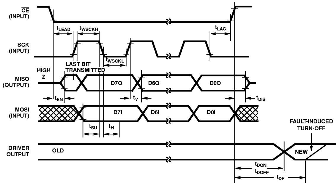
FIGURE 7B. SPI TIMING DIAGRAM
