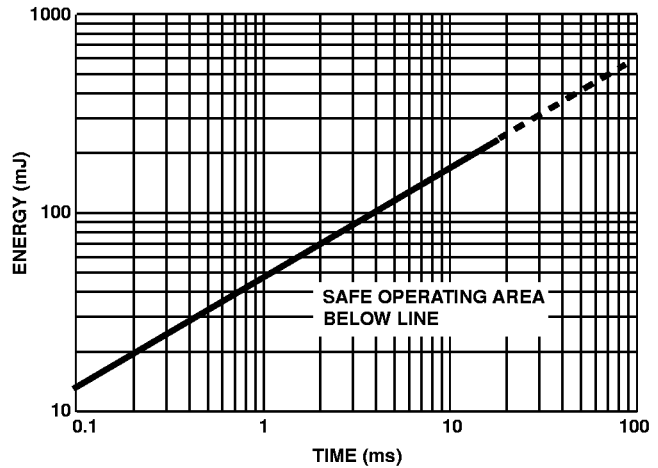
FIGURE 10. MAXIMUM SINGLE PULSE ENERGY SAFE OPERATING AREA FOR EACH CLAMPED OUTPUT DRIVER, T A = 25°C
