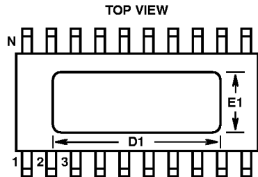
POWER SOP PACKAGE (HEAT SLUG SURFACE IS ELECTRICALLY FLOATING)
