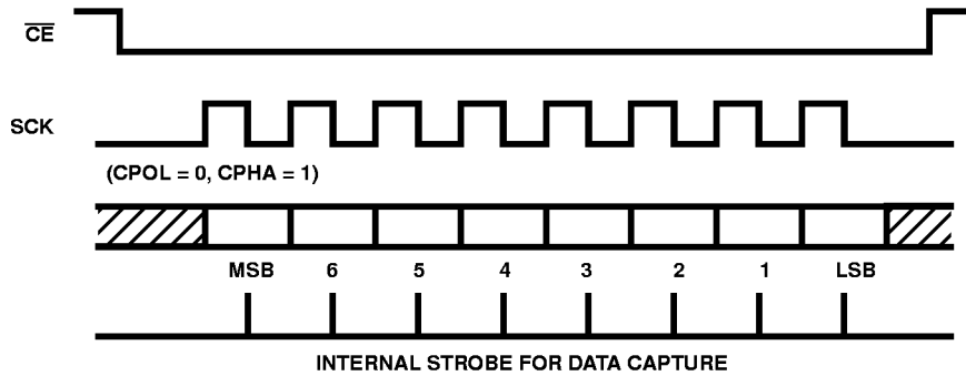
FIGURE 7A. DATA AND CLOCK TIMING DIAGRAM
