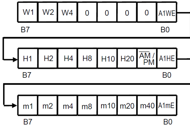
INT register 1
