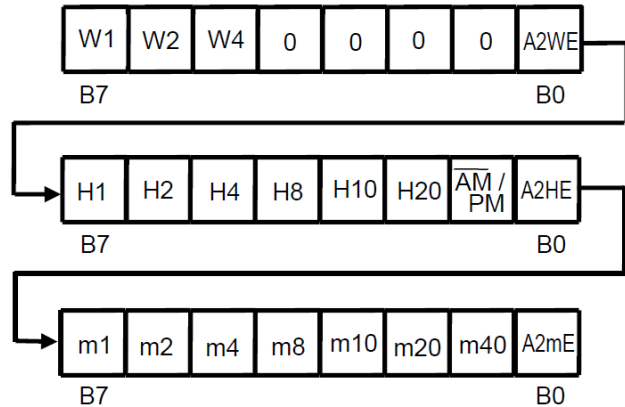
INT register 2
