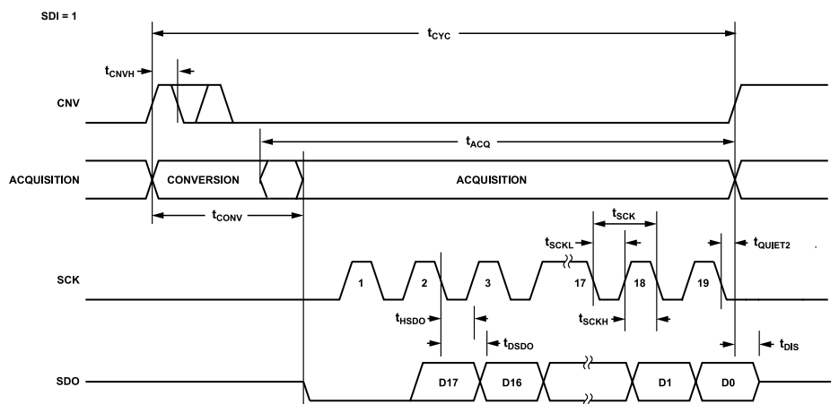
Figure 61. \overline{\text{CS}} Mode, 3-Wire with Busy Indicator Serial Interface Timing Diagram (SDI High)
