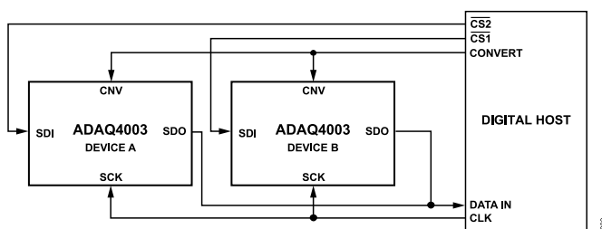
Figure 64. \overline{\text{CS}} Mode, 4-Wire Without Busy Indicator Connection Diagram
