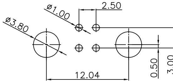
PC.BOARD LAYOUT
